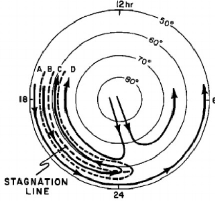
Figure 2-3: Diagram of the stagnation mechanism copied from (Spiro et al., 1978)
