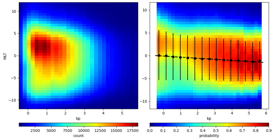
Figure 4.10: Motion of MIT towards pre-midnight with increased Kp
