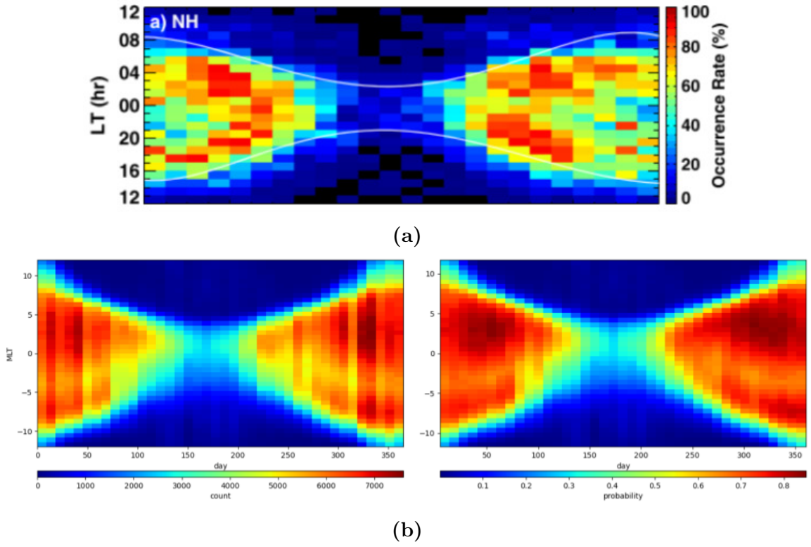
Figure 4.4: MIT occurrence rate in season - MLT bins. (a) (Aa et al., 2020), white lines indicate average solar terminator at 60^\circ MLat. (b) MIT season-MLT distribution and occurrence probability on the left and right respectively.
