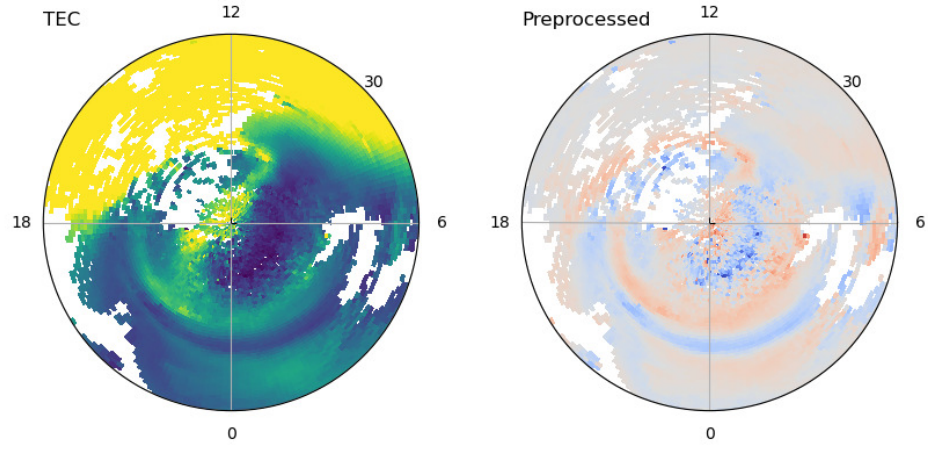
(a) Input (left) and output (right) to the preprocessing step: TEC and pre-processed vector, respectively
