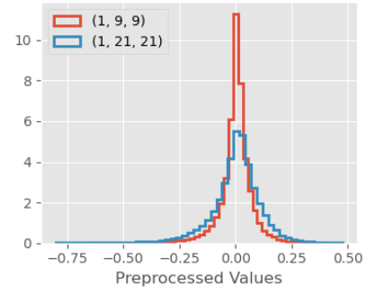
(c) Distributions of preprocessed values with different filter sizes
