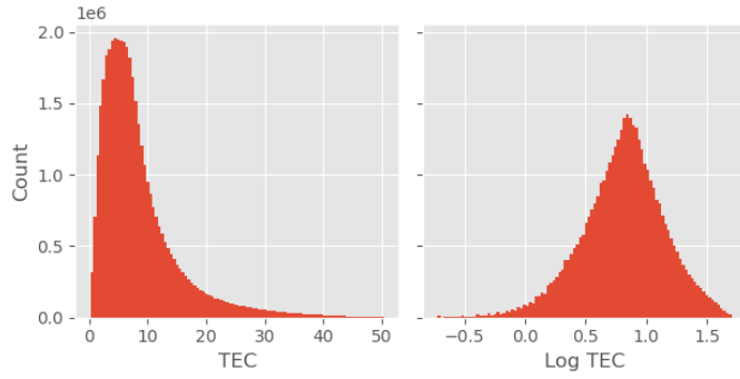
(b) Distributions of TEC (left) and Log TEC (right)
