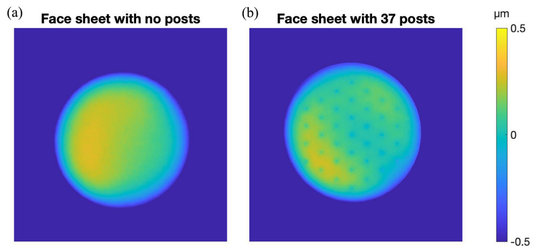
Figure 8. Surface topography maps of two 12 mm diameter edge-supported face sheets fabricated from the 10 \mu\text{m} thick device layer of a silicon-on-insulator wafer. (a) Face sheet with no posts. Deviation from flatness over the entire surface was 250 nm-rms. Local deviation from flatness in a 1.5 mm square region was 5 nm-rms. (b) Face sheet with 37 posts etched into the handle layer. Deviation from flatness over the entire surface was 180 nm-rms. Local deviation from flatness in a 1.5 mm square region was 29 nm-rms.
