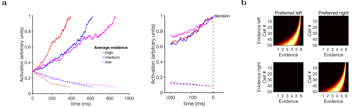
Figure 4. The Laplace transform and the inverse transform capture key findings from the neurobiology of evidence accumulation. a. The Laplace transform is shown for one value of s in a simulated random dot motion experiment. In this simulation, \alpha_L(t) was set at each moment to a normally-distributed random variable with a mean that differed across condition. In the solid curves, the mean was greater than zero; in the dashed curves the mean was less than zero for \alpha_L(t) (and thus greater than zero for \alpha_R(t) ). On the left we see that the firing rate grew with time after information began to accumulate; the rate and direction of accumulation depended on the mean of the random variable. When aligned to the time of response (right), firing rate showed a tight coupling. If we changed the value of s , we would have observed the same qualitative behavior, but with different rates of accumulation and more or less curvature on average. Compare to Fig. 1a. b. Heatmaps for neurons participating in the inverse Laplace transform. Each line is the firing rate of a neuron. Neurons participating in \tilde{f}_L are shown on the top; neurons participating in \tilde{f}_R are shown on the bottom. On the left the firing rate is shown as a function of evidence (confounded with time) when there is consistent evidence for the left option. On the right, the activation is shown when there is consistent evidence for the right option. Compare to Fig. 1b.
