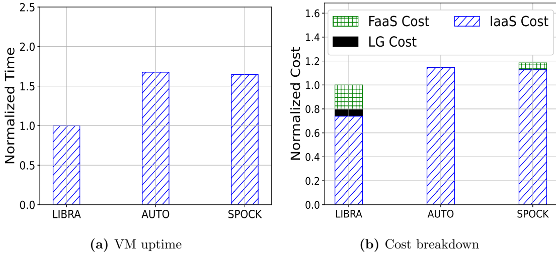
Figure 6-7: VM usage and cost breakdown
