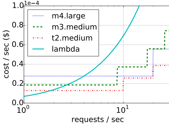
(b) Cost at Request Memory=512MB
