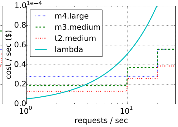
(c) Cost at Request Memory=3008MB
