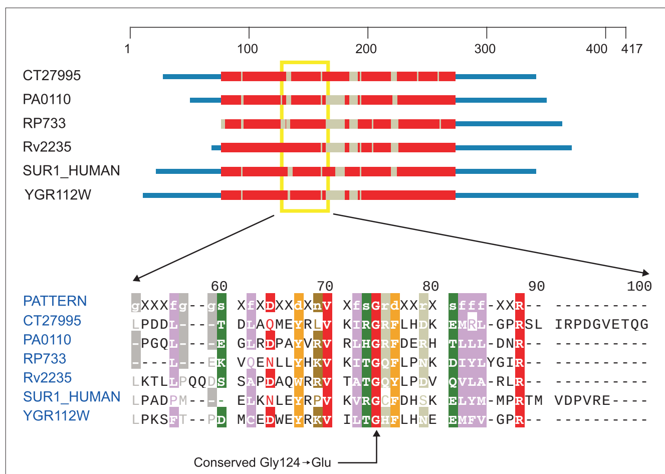
Figure 6 Domain diagram and partial alignment for surfeit locus protein I (SURFI). The column indicated by an arrow at the bottom corresponds to position 124 of SUR1_HUMAN. Sequences come from Drosophila melanogaster (CT27995), Pseudomonas aeruginosa (PA0110), Rickettsia prowazekii (RP733), M. tuberculosis (Rv2235), H. sapiens (SUR1_HUMAN) and S. cerevisiae (YGR112W). Colors are as in Figure 1.
