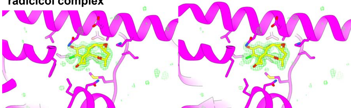
CMLD013075 complex
