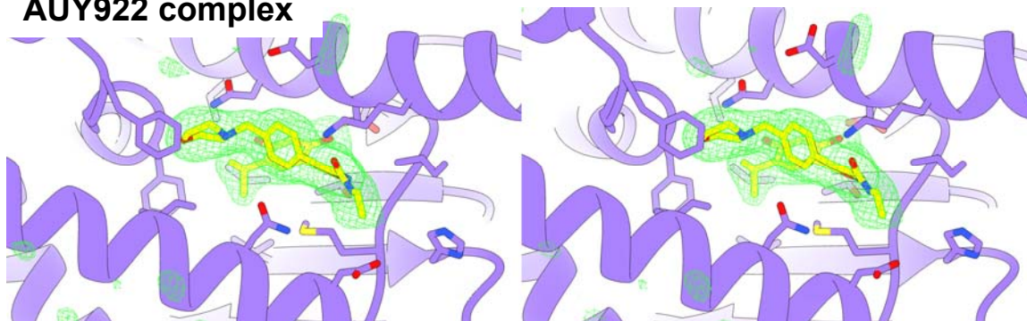
AUY922 complex
