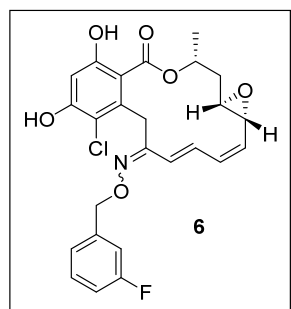
(1aR,2Z,4E,14R,15aS)-8-chloro-6-(((3-fluorobenzyl)oxy)imino)-9,11-dihydroxy-14-methyl-1a,6,7,14,15,15a-hexahydro-12H-benzo[c]oxireno[2,3-k][1]oxacyclotetradecin-12-one (6). Obtained
