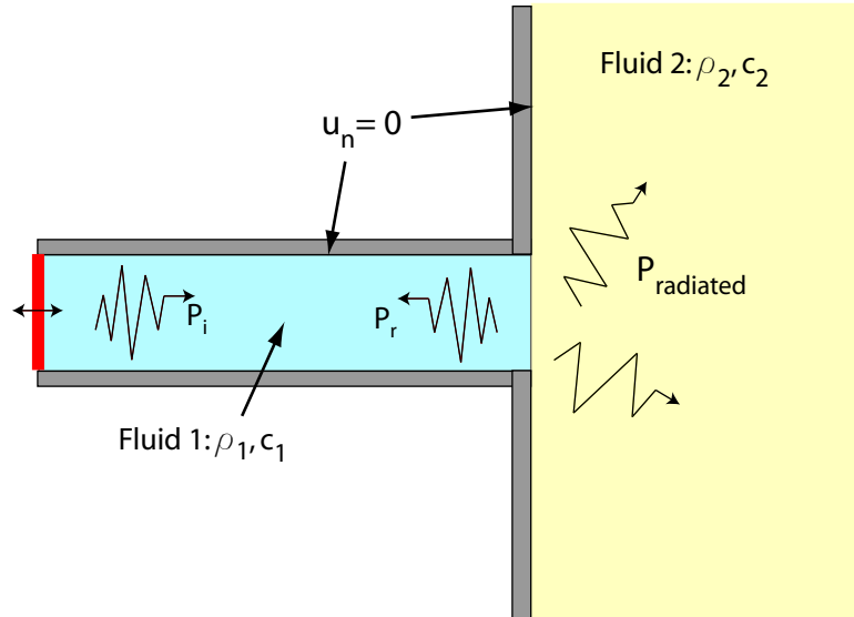
Figure 2.1: The baffled sound hard tube. A pressure wave traveling from the sound source at left hits the baffled opening. Some of the energy is reflected and some is radiated into the fluid outside the tube.
