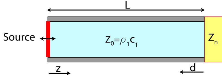
Figure 2.4: Tube terminated with unknown impedance, Z_n .
