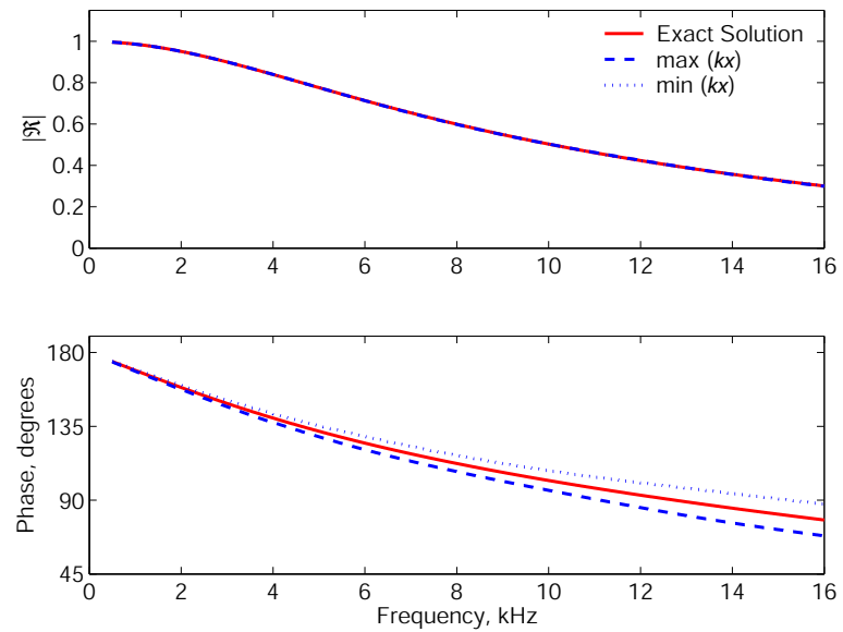
Figure 3.26: Effect of uncertainty in measured TFM input parameters for a simulated baffled tube opening.
