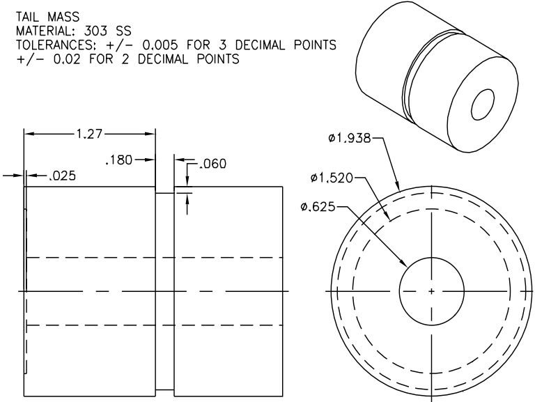
Figure D.4: Dimensioned drawing of source tail mass
