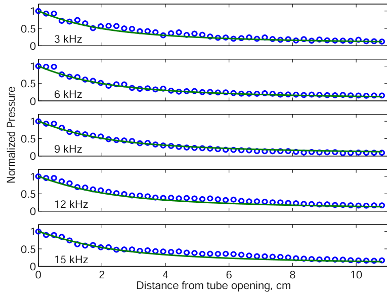
Figure 4.7: Radiated pressure profile as a function of distance from the tube opening. Measurements (open circles) are compared with the theoretical result (solid line).
