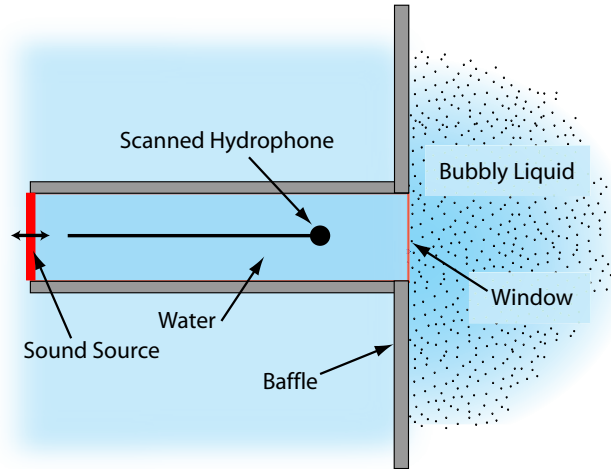
Figure 1.3: The submersible, baffled water-filled impedance tube.
