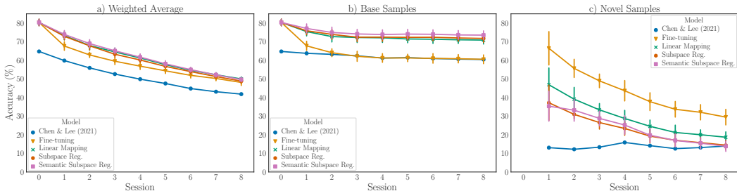
Figure 2: Multi-Session FSCIL accuracy (%) results on miniImageNet . In the first session 0, there are a total of 60 classes ( base ). Every session following the first one introduces 5 novel classes with 5 labeled samples from each. Each session provides accuracy over all classes that were seen thus far. Weighted average is the weighted combination of novel and base accuracies with respect to the number of classes in each category. Error bars are standard deviation (95% CI). In accordance with Chen & Lee (2021) we preserve only one sample per class from previous classes and append them to the support set during fine-tuning (+M variant). Regularization based approaches i.e. subspace regularization , semantic subspace regularization and linear mapping consistently outperform previous benchmarks on average.
