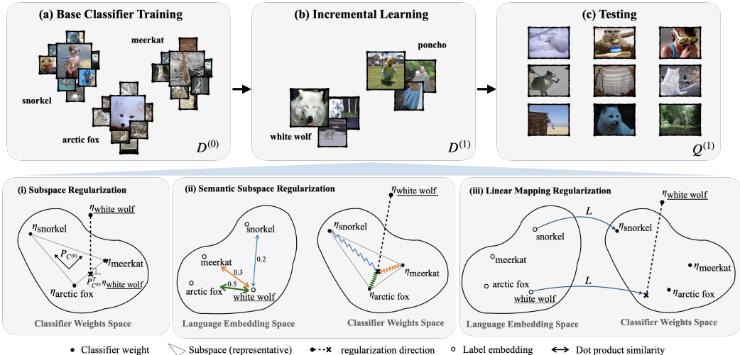
Figure 1: Few-shot class incremental learning: (a) A base classifier is trained on a large dataset ( D^{(0)} ). (b) This classifier is extended to also discriminate among a set of new classes with a small number of labeled examples ( D^{(1)} ). (c) Models are evaluated on a test set that includes all seen classes ( Q^{(1)} ). This paper focuses on extremely simple, regularization-based approaches to FSCIL, with and without side information from natural language: (i) We regularize novel classifier weights toward the shortest direction to the subspace spanned by base classifier weights. (ii) We regularize novel classifiers pulling them toward the weighted average of base classifiers where weights are calculated using label/description similarity between novel and base class names or one-sentence descriptions. (iii) We learn a linear mapping L between word labels and classifier weights of the base classes. Later, we project the novel label white wolf and regularize the novel classifier weight \eta_{white\ wolf} towards the projection.
