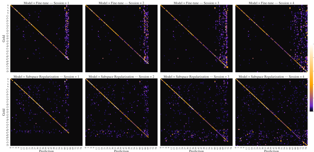
Figure 3: Simple fine-tuning (top) vs. subspace regularization (bottom) predictions without memory across the first four incremental sessions of miniImageNet . In the x - and y -axes, we present predictions and gold labels ranging from 0 to 79 where the first 60 are base classes. The number of classes grows by 5 every session starting from 60 up to 80. Brighter colors indicate more frequent predictions. Note that simple fine-tuning entails bias towards the most recently learned classes (top row) whereas addition of subspace regularization on the novel weights remedies the aforementioned bias; resulting in a fairer prediction performance for all classes.
