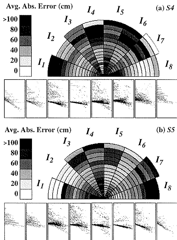
Figure 4: Predictive error of the raw sonars. (a) S4 , and (b) S5 . Semicircular plots show average absolute error level in each radial/distance bin (bins not shown were not sampled in data collection). Small dot plots show error for each datum collected, one plot for each of the eight angles of approach. Y axis thus shows predicted distance minus recorded, and is in the range [-200, 300] (cm). The X axis range is from [0, 325] (cm).
