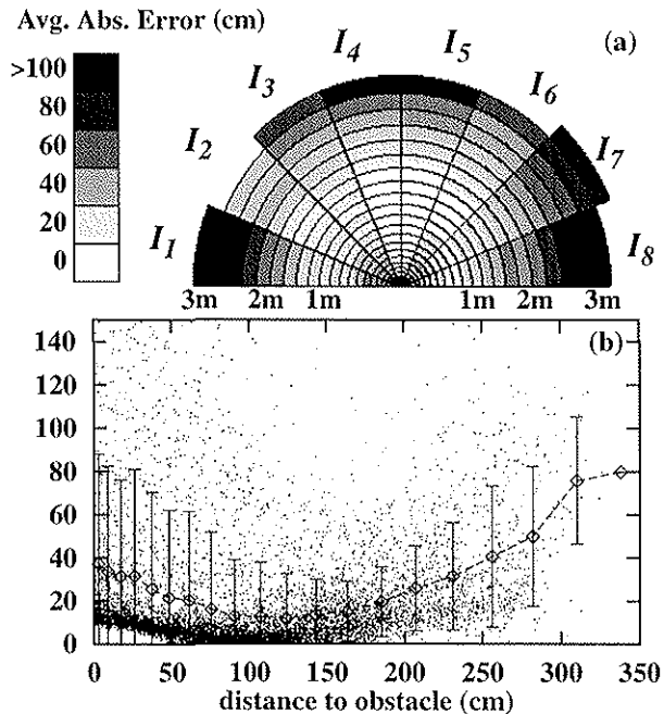
Figure 5: Predictive error of the \min(S4, S5) model. (a) Average absolute error in each sampling bin. Model predictions of distance are accurate at short distances and head-on approaches, but performance is impaired at longer distances or more oblique angles of approach (b) Absolute error by distance. Dots show absolute predictive error for each datum, dotted line shows average absolute error for each distance bin, and error bars indicate one standard deviation.
