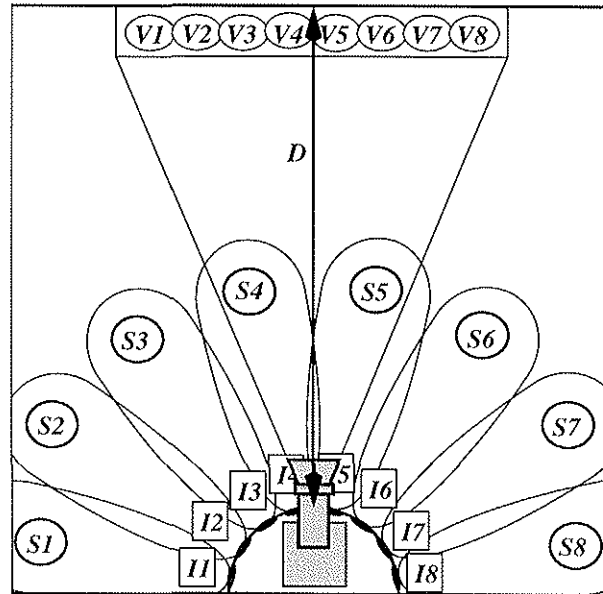
Figure 1: Overhead view of the B14 robot, showing its ranging sensors. Closest to the robot are infrared sensors, labeled I1-I8. These detect obstacles at close range, and specify the angle at which the obstacle is encountered. Sonars are labeled S1-S8 (beams emanating radially from robot). A camera is mounted on top of the robot, and provides gray-scale images. An edge detection algorithm is applied to these images, yielding visual sonar , a distance metric depicted as sensors V1-V8 (See Fig. 2). Odometry provides the distance D to the nearest obstacle.
