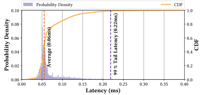
(b) UKL Echo server
