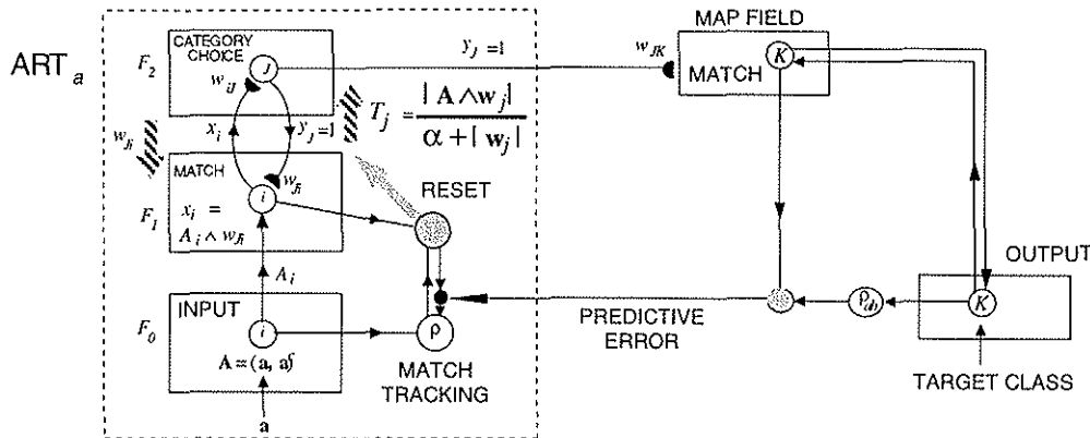
Figure 1: A fuzzy ARTMAP network for classification.
