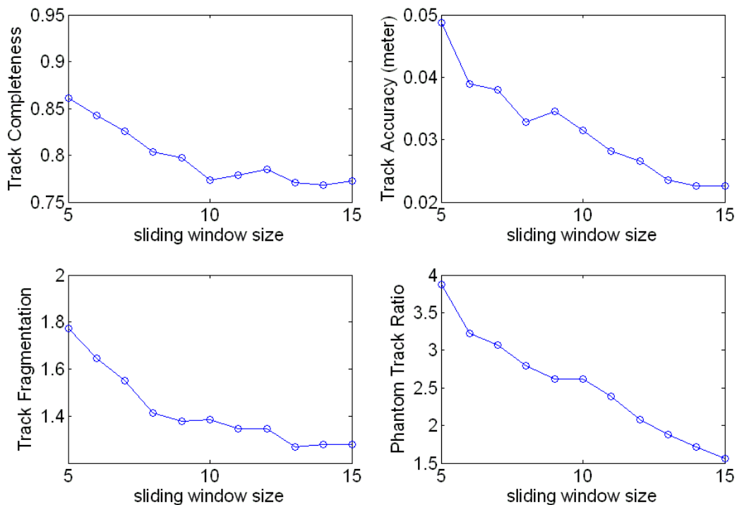
Figure 5. Tracking performance of the RECONSTRUCTION-TRACKING METHOD with different sliding window sizes T .
