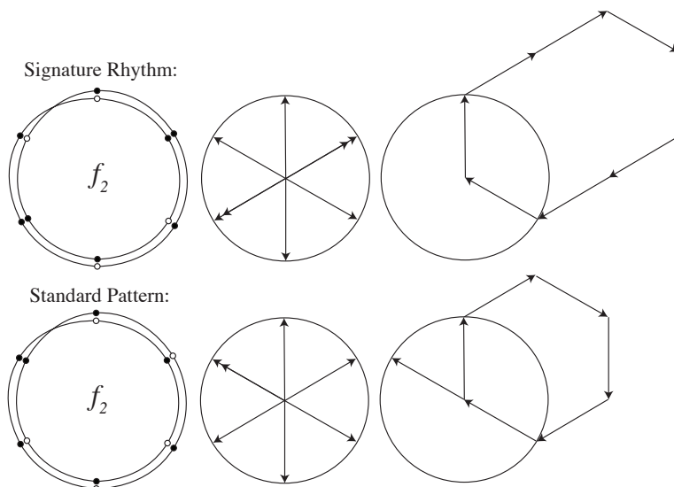
Figure 6: Calculation of f_2 for Reich’s signature rhythm and the standard pattern
