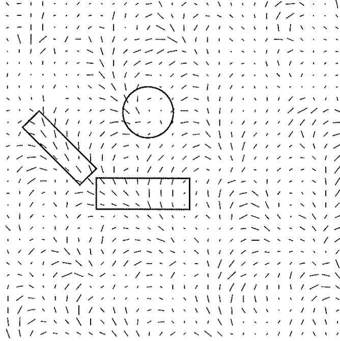
Figure 11. Orientation Map: Subset of the simulated binocular orientation map. Key features of the biological orientation maps are present here: (a) singularities; (b) linear zones; (c) fractures.
