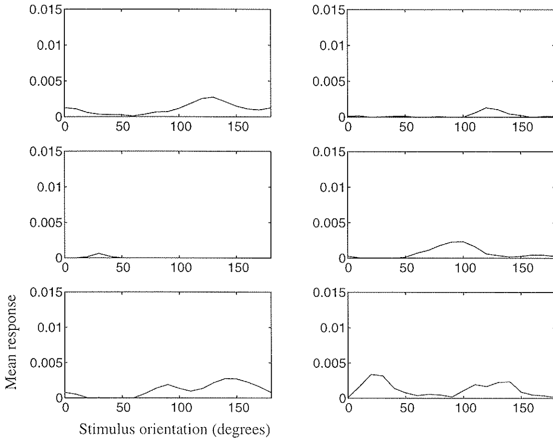
Figure 14. Simple Cell Orientation Tuning: Model cell response plotted against test bar orientation for six characteristic model simple cells.
