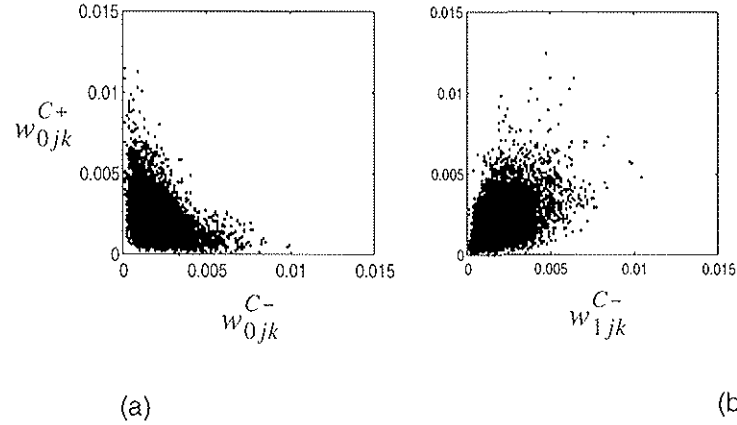
Figure 18. Simple Cell Opponency: (a) Value of each weight w_{0jk}^{C+}(l, m) from the ON LGN to units x_{0jk} versus weight w_{0jk}^{C-}(l, m) from the OFF LGN. They are clearly anti-correlated. (b) Value of each weight w_{0jk}^{C+}(l, m) from the ON LGN to units x_{0jk} versus weight w_{1jk}^{C-}(l, m) from the OFF LGN to the antagonistic units x_{1jk} . Because of the opponency developed by the model cells, each cell has an ON region that is correlated with the OFF region of its opponent.
