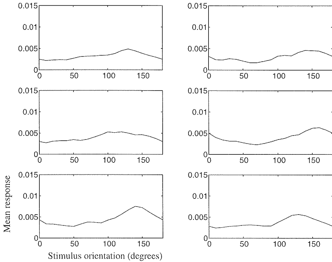
Figure 15. Complex Cell Orientation Tuning: Model cell response plotted against test bar orientation for six characteristic model complex cells.
