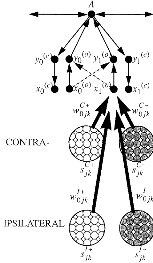
Figure 19. Two-Dimensional Model: In addition to two cortical dimensions, inputs from both eyes are simulated. Contralateral (C) and ipsilateral (I) ON and OFF LGN cells project via weighted retinotopically arranged pathways to each x unit. The two-dimensional model approximates the dynamical system as a progression of open ( o ) and closed
