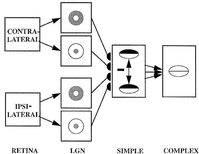
Figure 1. Model Overview: Inputs to the two eyes project forward to ON and OFF cells in the LGN. ON and OFF LGN cells from both eyes converge on cortical simple cells, which are arranged into mutually inhibitory pairs. The simple cells in turn project forward to complex cells. Model complex cells thus derive their orientation tuning from the underlying simple cells
