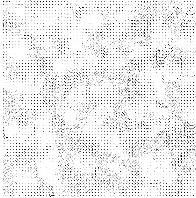
Figure 12. Orientation Preference and Ocular dominance maps: Orientation preference at each position is indicated by a line segment at the preferred orientation with length proportional to orientation selectivity. Regions dominated by the contralateral eye are colored white, regions dominated by the ipsilateral eye are grey.
