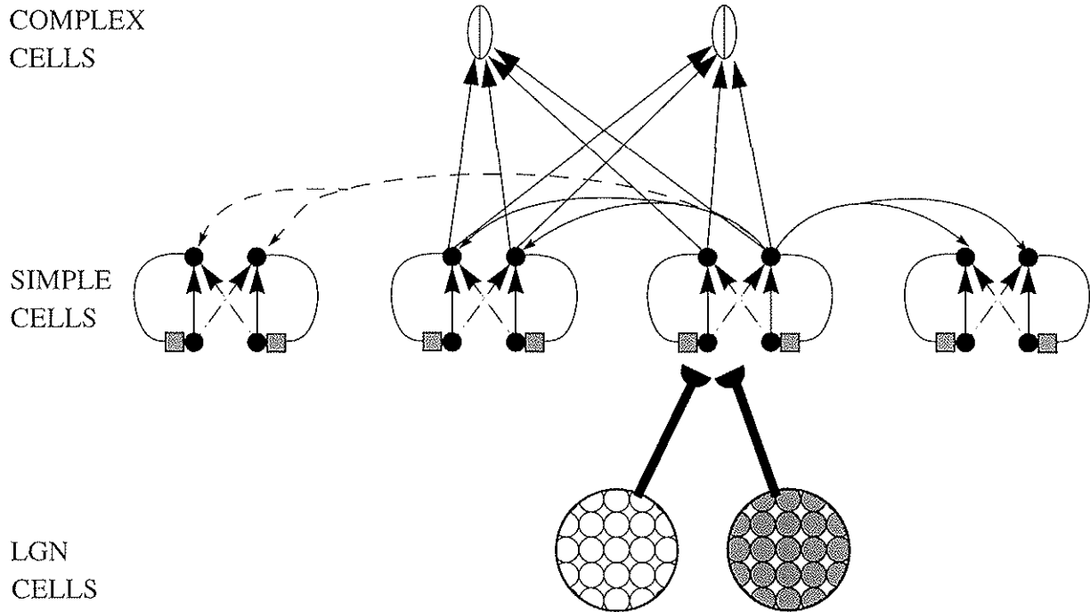
Figure 4. Lateral Connectivity and Complex Cells: Distance dependent connection strengths between y units realize a band pass filter. Complex cells respond according to the weighted sum of simple cell responses.
