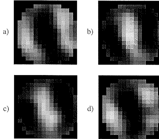
Figure 7. Opponency of Final Weight Profiles: Self organization leads to the development of opposite polarity ON and OFF weight profiles in opponent simple cells. Weight images after 6000 training presentations: (a) w_0^+(1, 24) ; (b) w_0^-(1, 24) ; (c) w_1^+(1, 24) ; (d) w_1^-(1, 24)
