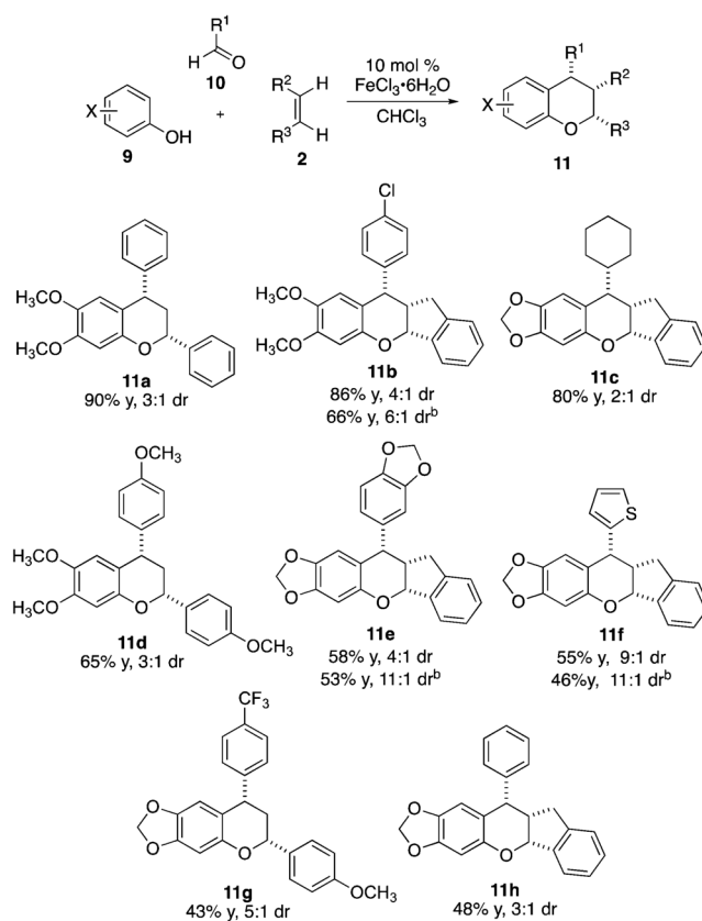
Figure 3. Multicomponent condensation reaction with aldehydes, phenols, and olefins. a a Reaction conditions: 2.0 mmol of phenol, 2.0 mmol of aldehyde, and 1.0 mmol of dienophile, 0.5 M with respect to dienophile and 10 mol % \text{FeCl}_3 \cdot 6\text{H}_2\text{O} with respect to phenol; isolated yields; diastereomeric ratio determined by ^1\text{H} NMR; detailed experimental conditions are provided in the Supporting Information. b Yield and dr after trituration with hot hexanes.
