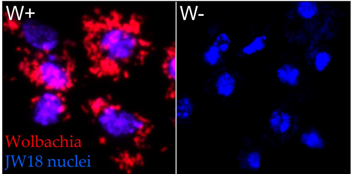
Figure 4.1: JW18 cells stained for Wolbachia using FISH.
