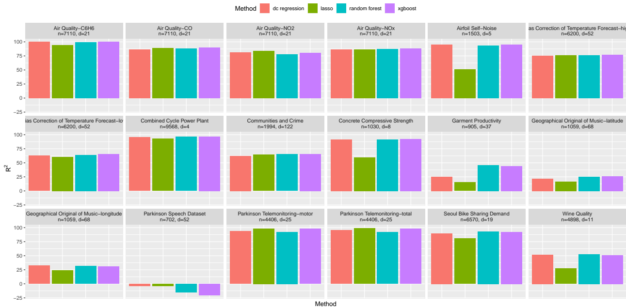
Figure 1. Regression results on UCI datasets
