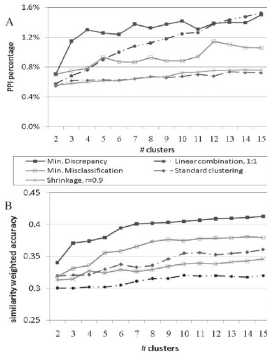
Fig. 2. Clustering performances as a function of the number of clusters: average accuracy over 10 experiments. (A) Overall PPI percentage in the obtained clusters. (B) The 5-fold cross-validation tests, sw-accuracy.
