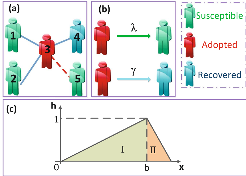
Figure 1. (a) Illustration of social contagions on complex networks. (b) Schematic of information transmission from the adopted individual to his each susceptible neighbor with probability \lambda and state change from being adopted to recovered with probability \gamma . (c) Tent-like behavior adoption probability. Notations b and x indicate local trend imitation capacity and the ratio of adopted informants, respectively. In region I, the adoption probability increases with x . In region II, the adoption probability decreases with x .
