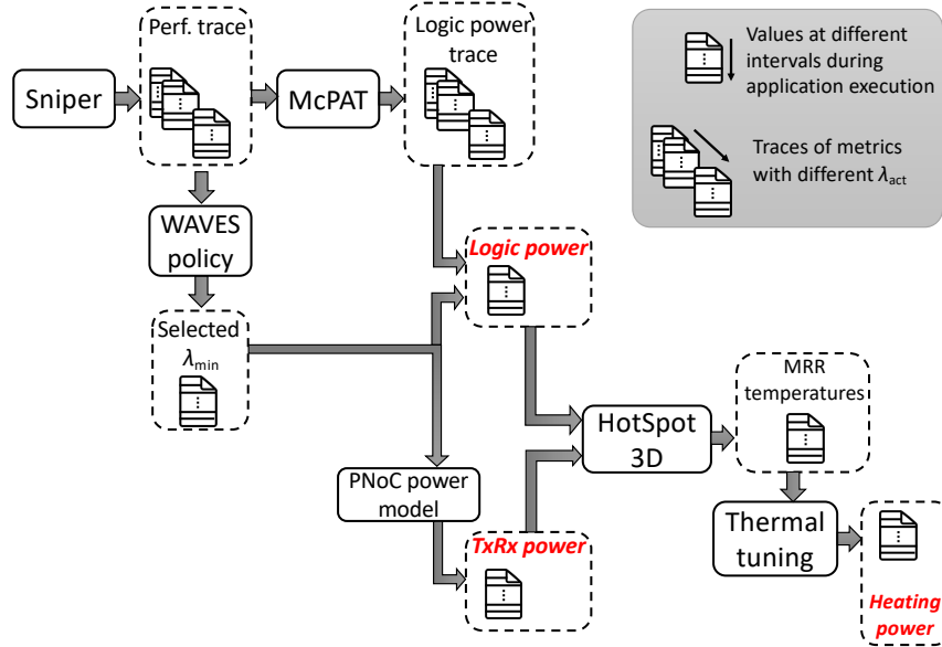
Figure 3-2: Simulation framework for modeling performance, power and temperature of POPSTAR .
