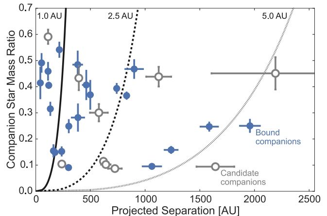
FIG. 6.— For each companion in our survey sample, we plot the companion’s mass and projected separation. Each point represents the weighted average from all observations in Table 6. The lines represent the minimum companion mass necessary to excite Kozai-Lidov oscillations at a timescale short enough to overcome general relativity pericenter precession. These representative lines assume a primary stellar mass of 1.0 M_\odot , a planetary mass of 1.0 M_{\text{JUP}} , a circular planetary orbit and a stellar companion eccentricity of 0.5. The three lines (solid, dashed, and dotted) represent the difference in pericenter precession timescales for a hot Jupiter starting at 1 AU, 2.5 AU and 5 AU, respectively. Companions must be above and to the left of these lines to overcome general relativity pericenter precession timescales.
