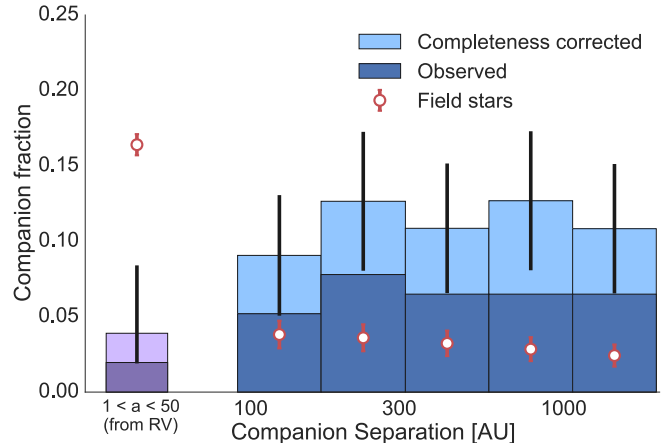
FIG. 9.— Companion fraction as a function of companion separation, in logarithmic bins, for targets in the completeness corrected survey sample (light blue), the uncorrected survey sample (dark blue), and the field star sample (open red symbols). The leftmost bin represents the corrected (light purple) and uncorrected (dark purple) companion fraction from 1 AU to 50 AU, computed from long term RV sensitivity surveys. The field star values (open red circles) are from Raghavan et al. (2010) and are also completeness corrected.
