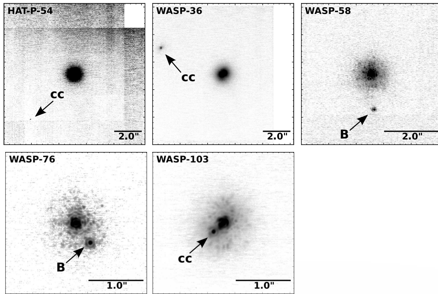
FIG. 2.— Median-stacked K band image for each detected candidate multi-stellar system presented in this work, from our non-survey targets. Each image is oriented such that North points up and East to the left.
