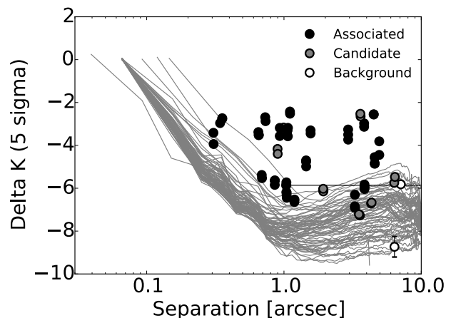
FIG. 5.— 5\sigma K band contrast curve computed from stacked images for all observed targets. The curve with the best contrast for each target is shown. For these curves, all companion stars are masked out. Detections of bound companions, candidate companions, and background objects as overplotted as filled black, grey, and open circles, respectively.
