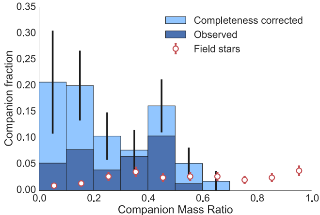
FIG. 8.— Companion fraction as a function of companion mass ratio for targets in the completeness corrected survey sample (light blue), the uncorrected survey sample (dark blue), and the field star sample (open red symbols). The field star values (open red circles) are from Raghavan et al. (2010) and are also completeness corrected.
