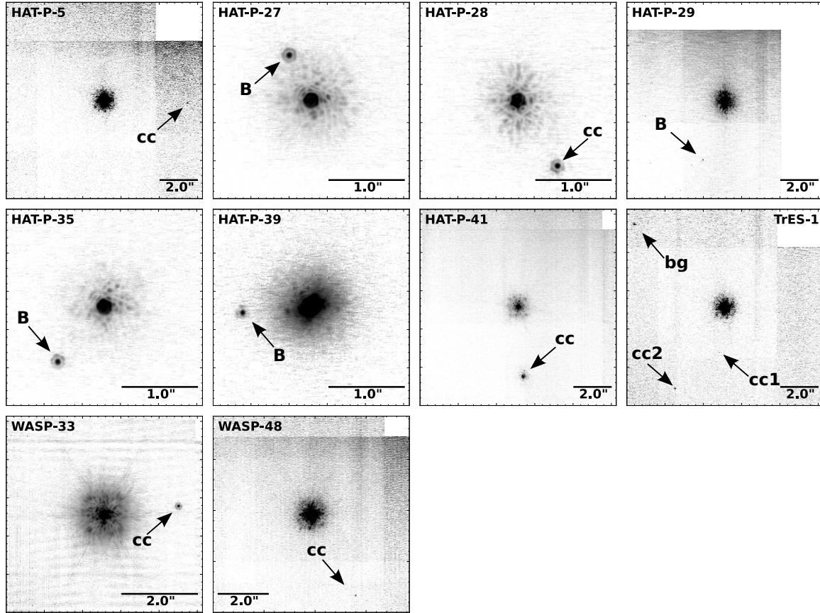
FIG. 1.— Median-stacked K band image for each detected candidate multi-stellar system presented in this work, from our survey targets. Each image is oriented such that North points up and East to the left.
