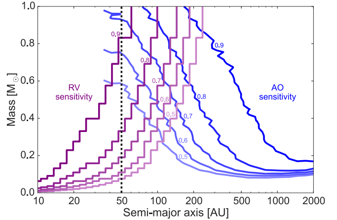
FIG. 7.— Contours of overall sensitivity to stellar companions from long term radial velocity surveys (purple) and our AO survey (blue). These sensitivities are averaged over all targets and computed for a typical 1 M_\odot target. The dashed line marks a semi-major axis of 50 AU.
