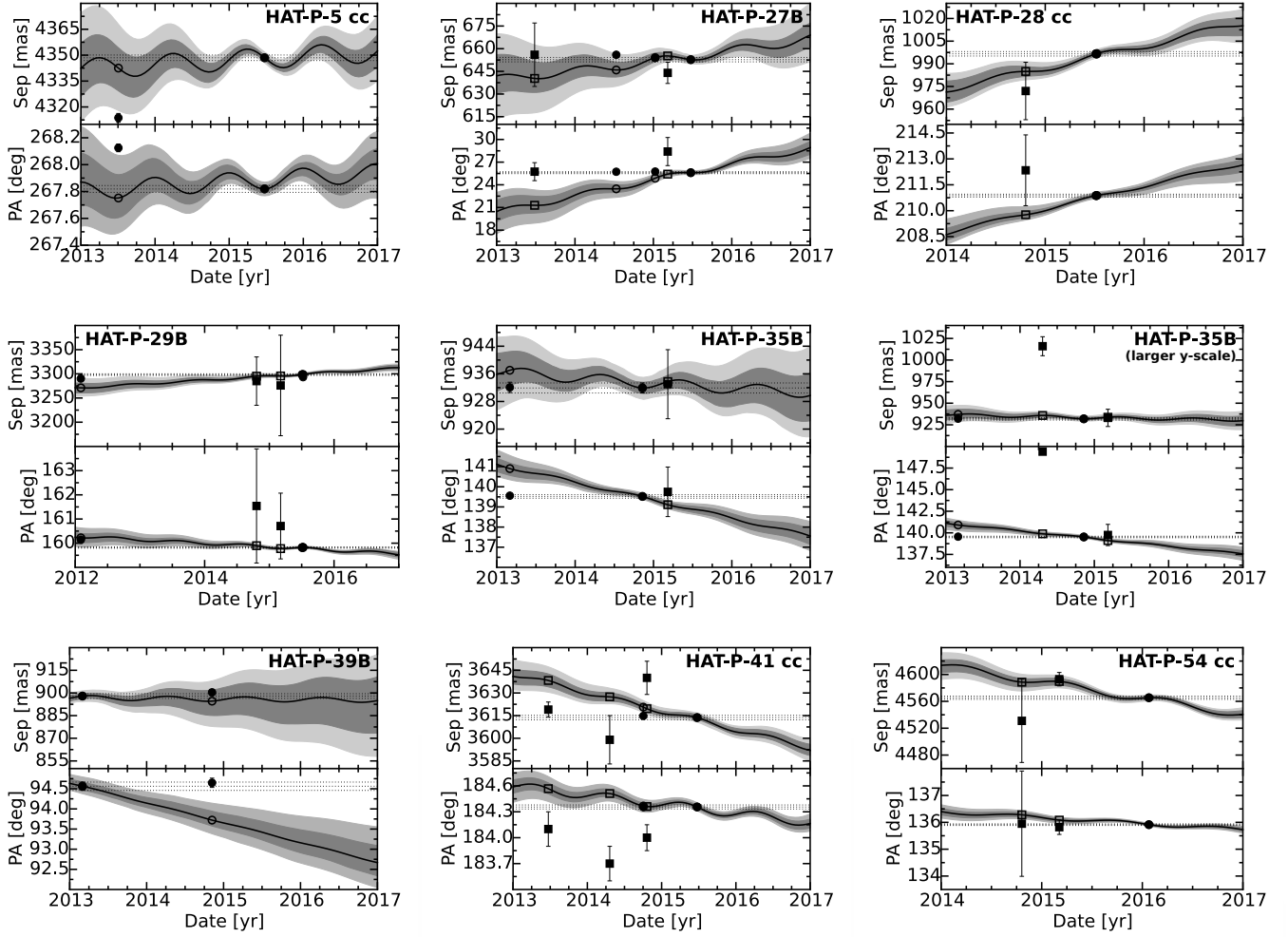
FIG. 3.— Common proper motion confirmation for each candidate companion. The top and bottom panels show the separation and position angle of a candidate companion relative to the primary star. The background track (solid line) starts at the observation with the smallest uncertainty in separation and position angle. The shaded region indicate the 68% and 95% confidence regions. We use uncertainties in our separation and position angle measurement as well as the uncertainties in the primary star’s celestial coordinates, proper motion, and parallax in our Monte Carlo routine to determine these confidence regions. The filled symbols show measured positions of companions (listed in Table 5 and open symbols show the expected position if the candidate object were a very distant background object. Circles are measurements from our campaign while squares are measurements from other studies. When the solid symbols and open symbols differ and when the measurement values are consistent with each other at all observation epochs, then we can conclude our detected object is a physically bound companion. Objects labeled as “B” have common proper motion, as “cc” are candidate companions and as “bg” are background objects. See Section 4. Continued in Figure 4.
