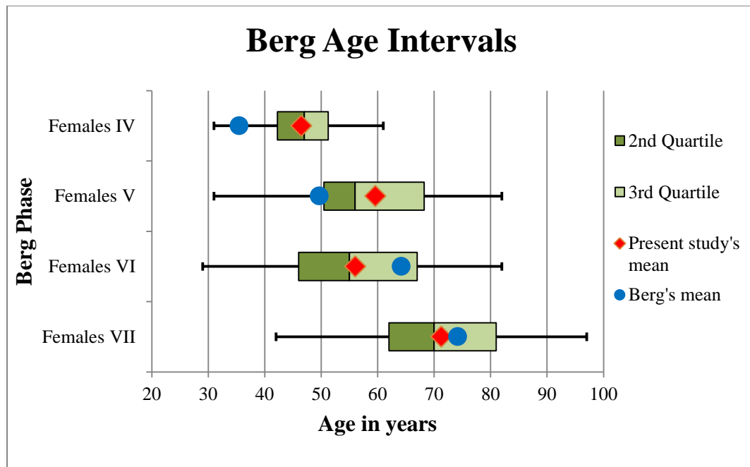
Figure 4.3. Box and whisker plot of the means and 100% age intervals calculated using the sampled individuals' Berg(2008) phase assignments. Red diamonds indicate the phase means calculated by the author while blue circles denote the phase means presented by Berg.
