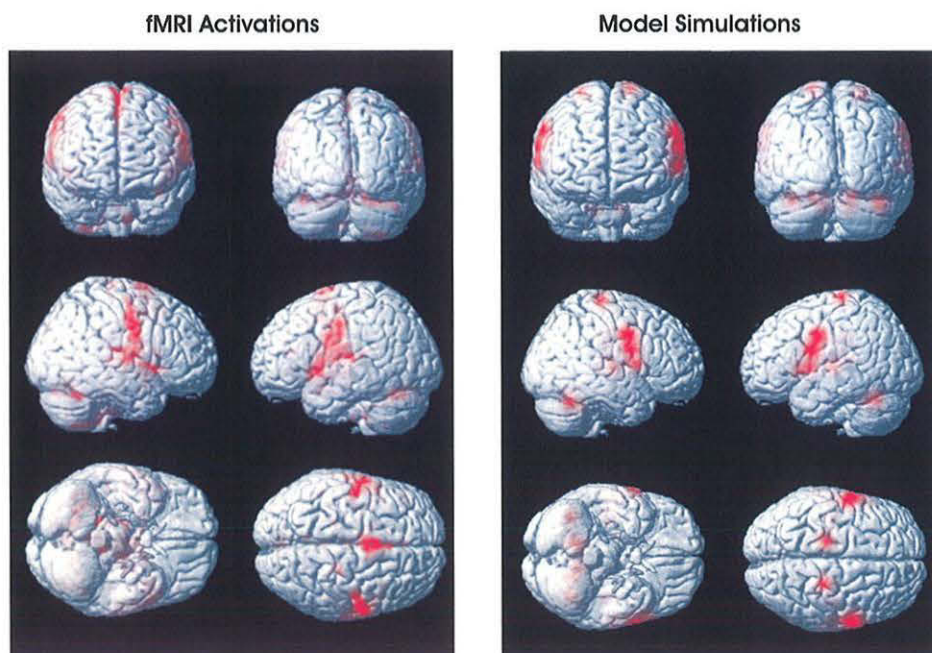
FIGURE 6. fMRI results (left) and model simulation results (right) for simple syllable production. Model activations were determined as follows. Positions in MNI space corresponding to different types of cells in the model were chosen as described in the text and summarized in Table 1. Model cell activities were normalized by the maximum possible activity of the cell. The resultant activity was convolved with an idealized hemodynamic response function (generated using default settings of the function 'spm_hrf' from the SPM toolbox). The convolved response was summed to generate a pseudo-BOLD value for each position. A brain volume was constructed with the appropriate values at each position, smoothed with a Gaussian kernel (FWHM=12mm). The resultant volume was then rendered using routines from the SPM
