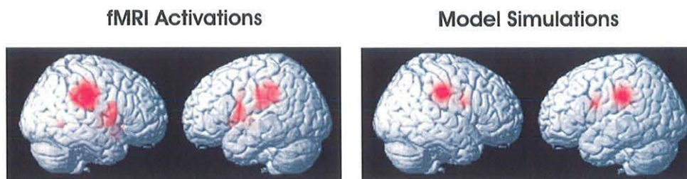
FIGURE 8. fMRI results (left) and model simulation results (right) for jaw-perturbed speech minus unperturbed speech (right panels). Model activations were determined as described in the caption of Figure 6.
