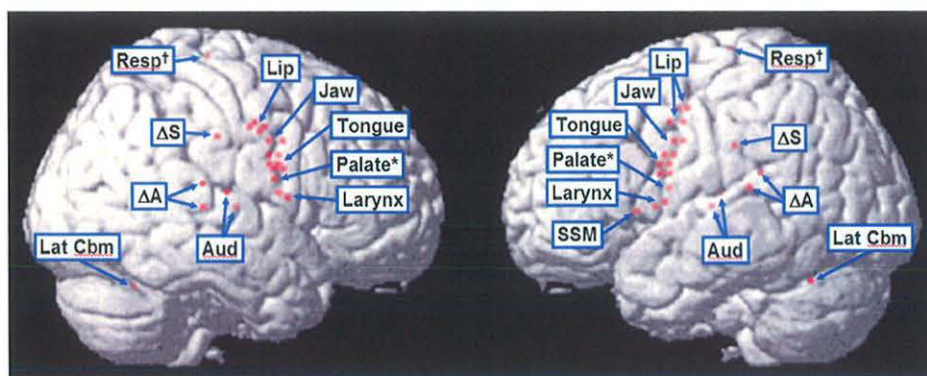
FIGURE 7. Rendered lateral surfaces of the SPM standard brain indicating locations of the model components as described in the text. Medial regions (anterior paravermal cerebellum and deep cerebellar nuclei) are omitted. Unless otherwise noted, labels along the central sulcus correspond to a motor (anterior) and a somatosensory (posterior) representation for each articulator. Abbreviation key: Aud = auditory state cells; ΔA = auditory error cells; ΔS = somatosensory error cells; Lat Cbm = superior lateral cerebellum; Resp = motor respiratory region; SSM = speech sound map. *Palate representation is somatosensory only. †Respiratory representation is motor only.
