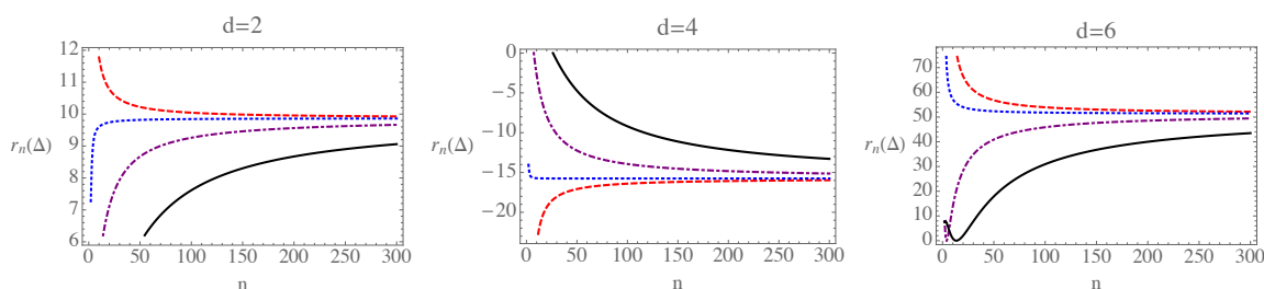
Figure 3. Ratio r_n(\Delta) for d = 2, 4, 6 (left, middle, right) at various \Delta : \Delta = -0.75 (red, dashed), \Delta = 1.25 (blue, dotted), \Delta = 7.25 (purple, dot-dashed), and \Delta = 26.25 (black, solid). The curves appear to converge to the same value at infinite n .
