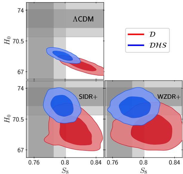
FIG. 4: Posterior distributions of \Lambda CDM (top left), SIDR+ (bottom left), and WZDR+ (bottom right) fitted to \mathcal{D} vs. \mathcal{DHS} data sets.
