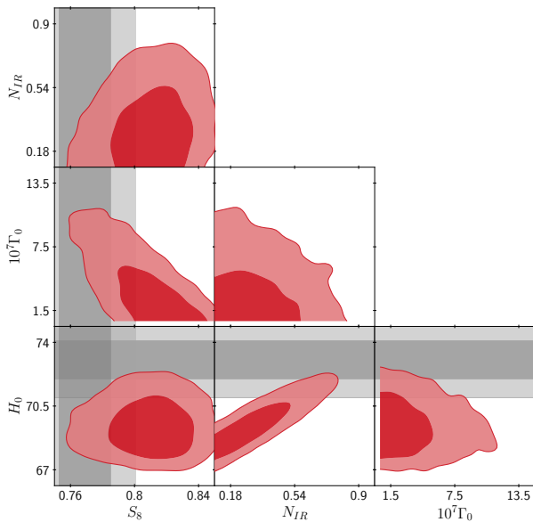
FIG. 3: Posterior distribution of WZDR+ fitted to the \mathcal{D} data set. The distribution shows a clear correlation between the model parameters N_{IR} and \Gamma_0 and the inferred quantities H_0 and S_8 .
