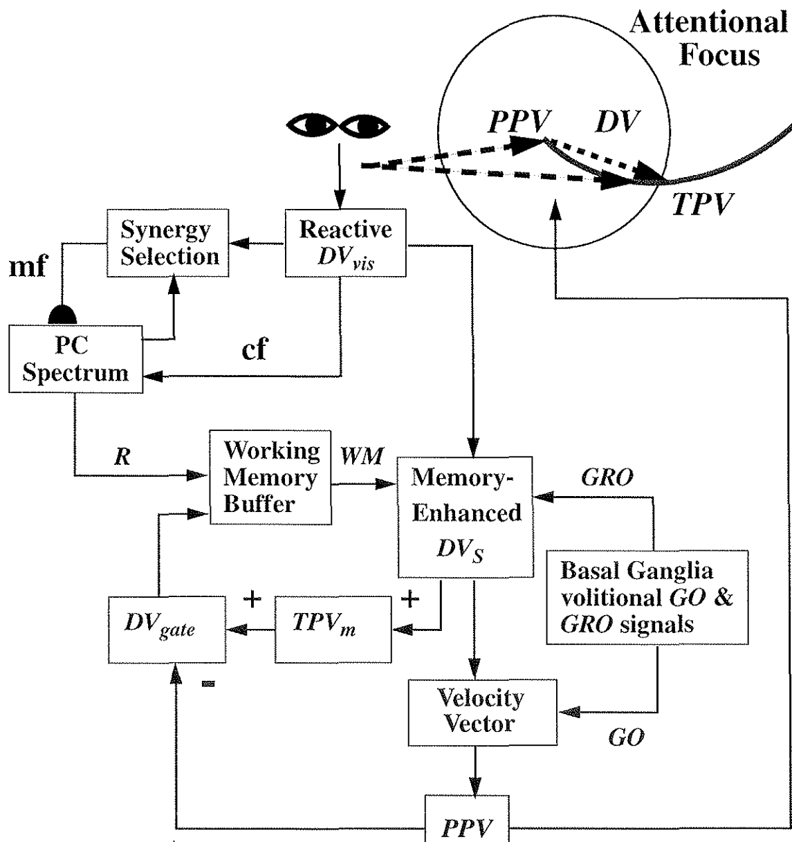
Figure 3.1. Diagram of the AVITEWRITE architecture. mf = mossy fiber; cf = climbing fiber; PC = Purkinje cell. See text for details.
