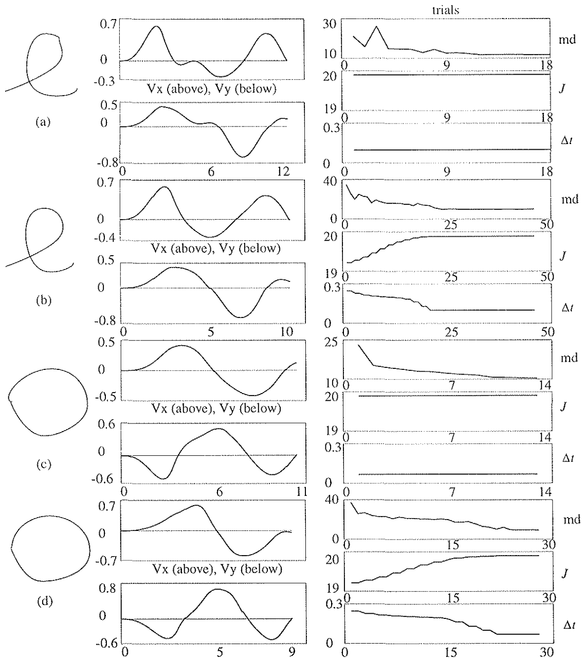
Figure 3.19. Letters learned with variable speed compared to learning at a constant, fast speed. In (a) and (c), the GO signal and spectral density were held constant ( J = 20 , \Delta t = 0.1 ). In (b) and (d), the GO signal and spectral density were incrementally increased every two trials according to the function in Figure 3.18 (starting at J = 19.25 , \Delta t = 0.25 ; ending at J = 20 , \Delta t = 0.1 ). The result was an increase in the range of movement durations, as seen in Table 3.1. (a) through (d): Left: Letter learned by AVITEWRITE; Middle: x and y velocity profiles, V_x , V_y ; Right: (top) trials versus movement duration (md); (middle) J over the course of learning; (bottom) \Delta t over the course of learning.
