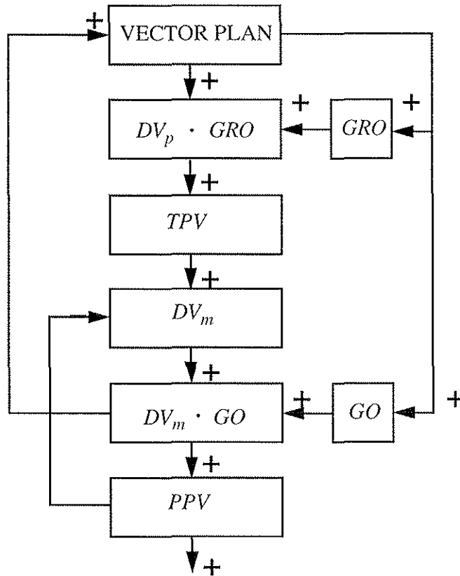
Figure 1.2. Schematic diagram of the VITEWRITE model of Bullock et al. (1993): A Vector Plan functions as a motor program that stores discrete planning vectors DV_p in a working memory. A GRO signal determines the size of script and a GO signal its speed of execution. After the vector plan and these will-to-act signals are activated, the circuit generates script automatically. Size-scaled planning vectors DV_p \cdot GRO are read into a target position vector ( TPV ). An outflow representation of present position, the present position vector ( PPV ), is subtracted from the TPV to define a movement difference vector ( DV_m ). The DV_m is multiplied by the GO signal. The net signal DV_m \cdot GO is integrated by the PPV until it equals the TPV . The signal DV_m \cdot GO is thus an outflow representation of movement speed. Maxima or zero values of its cell activations may automatically trigger read-out of the next planning vector DV_p . (Reproduced with permission from Bullock et al.,1993.)
