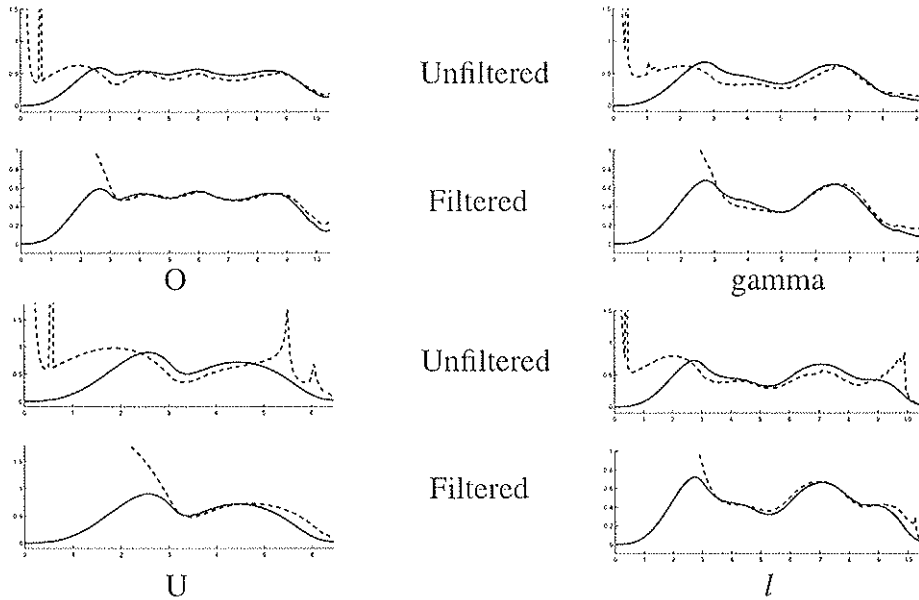
Figure 3.17. Two-Thirds Power Law predictions (dotted lines) of tangential velocity compared to the actual tangential velocity (solid lines) of AVITEWRITE for the letters O, U, gamma, and l . For each letter, the top panel shows the power law prediction calculated using the unfiltered model acceleration profile, and the bottom panel shows the prediction calculated using acceleration filtered with Equation (13). The values used for the constant of proportionality ( k ) in Equation (15) are as follows. O: 0.5; U: 0.6; gamma: 0.45; l : 0.5.
