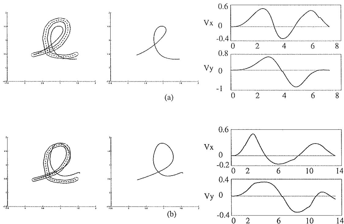
Figure 3.22. The effect of altering the spectral density of the letter l after learning with \Delta t = 0.1 : (a) Spectral density is increased by decreasing the time separation \Delta t between adjacent spectral components to 0.05. (b) Spectral density is decreased by increasing \Delta t to 0.13.
