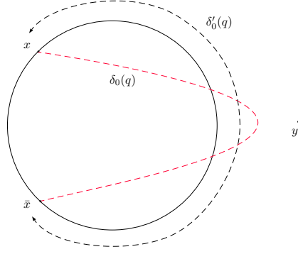
FIGURE 7. The deformed contour \delta'_0(q) .
