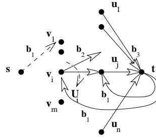
Fig. 14. Reduction from MAX-UNIQUES( k ) to Max-Min.
