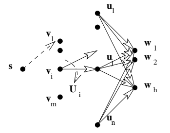
Fig. 15. Reduction from MAX-UNIQUES( k ) to Max-Sum.
