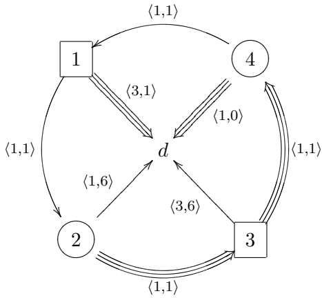
Figure 5: Solvable instance of \langle +, + \rangle -SPP with policies \langle \square, \circ \rangle .
