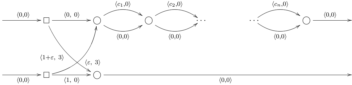
Figure 9: Routes through this graph correspond to solutions to the subset sum problem (with policies \langle \square, \circ \rangle ).
