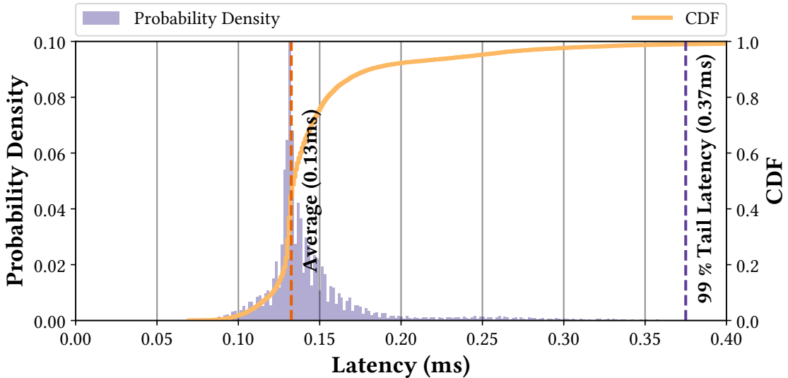
Figure 4-1: Probability density and CDF of latencies for the userspace echo server.
