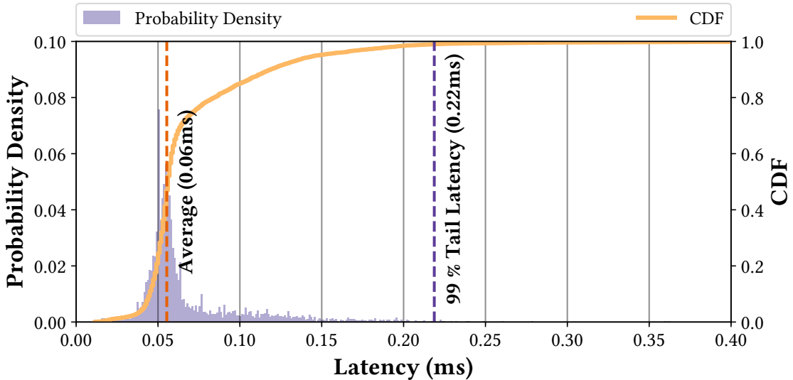
Figure 4.2: Probability density and CDF of latencies for the UKL echo server. The average latency of UKL echo server (0.06 ms) is less than half of that of the userspace case (0.13 ms), and the 99% tail latency for UKL (0.22 ms) is 41% faster than the userspace case (0.37 ms). See Figure 4.1.
