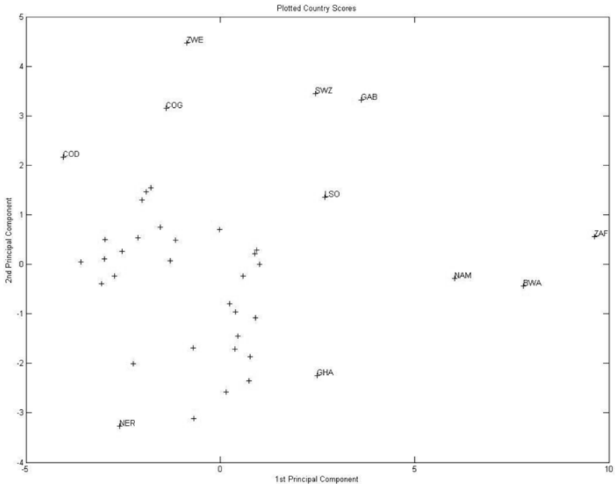
Figure 2: 1st and 2nd Principal Components Plotted Country Scores
