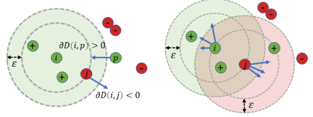
Figure 5. This figure complements Eq. 9. Part \textcircled{1} of the gradient (left) enforces correct ranking w.r.t. sample i . Part \textcircled{2} of the gradient (right) increases the distance between i and all samples in the neighborhood of j , and vice versa. As shown, sometimes this implies that samples with the same label are pulled apart. The k + \epsilon neighborhood as defined in Eq. 2 is shaded. k = 4 .
