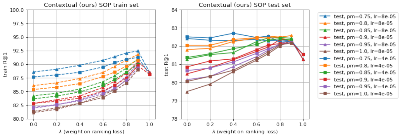
Figure 28. SOP R@1 results for our contextual loss function, with varying \lambda , learning rate, and positive margin on contrastive loss. We plot both train and test R@1 results. “lr” and “pm” in the legend stand for learning rate and positive margin \delta_+ , respectively.
