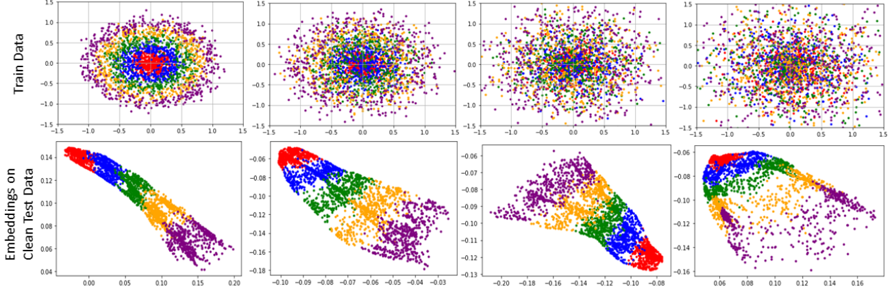
Figure 11. This figure justifies the non-standard approach of optimizing \mathcal{L}_1 (Eq. 32) by overriding the gradient of \theta . We generate synthetic 2-D data consisting of five concentric circles; each color represents a label. We use a standard three layer MLP with ReLU activations to output a 2D embedding. We train on increasingly noisy data and plot the resulting embeddings on clean data. We only sample 4 points per label per batch ( k = 4 ). \mathcal{L}_1 minimization results in reasonable embeddings despite its simplicity.
