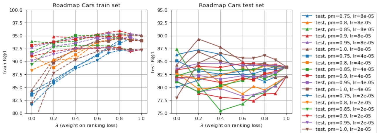
Figure 24. Cars R@1 results for Roadmap, with varying \lambda , learning rate, and positive margin on contrastive loss. We plot both train and test R@1 results. “lr” and “pm” in the legend stand for learning rate and positive margin \delta_+ , respectively.
