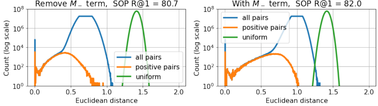
Figure 12. This figure justifies the M_- term in Eq. 24. The left plot shows the distribution of distances between pairs in normalized embedding space when we only optimize M_+ ; the right plot shows the same when we optimize both M_- and M_+ . A uniformly distributed embedding space has an average pair-wise distance of \sqrt{2} because most directions are orthogonal in high dimensions. This is indicated by the green distribution. Clearly, more of the embedding space is utilized when we optimize both M_- and M_+ .
