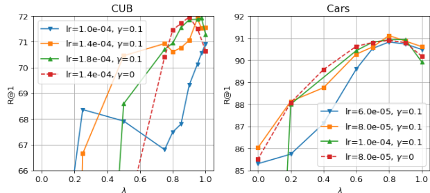
Figure 7. Ablation results. We test the contribution of each component in Eq. 6 by trying different values for \lambda and \gamma on CUB and Cars. The dashed line indicates results without the similarity regularizer ( \gamma = 0 ). The three different marker symbols represent different learning rates. We show results for different learning rates because the optimal learning rate varies with \lambda . Observe that the optimal R@1 is always achieved by a combination of \mathcal{L}_{\text{contrast}} and \mathcal{L}_{\text{context}} . The similarity regularizer is sometimes helpful, but never detrimental.
