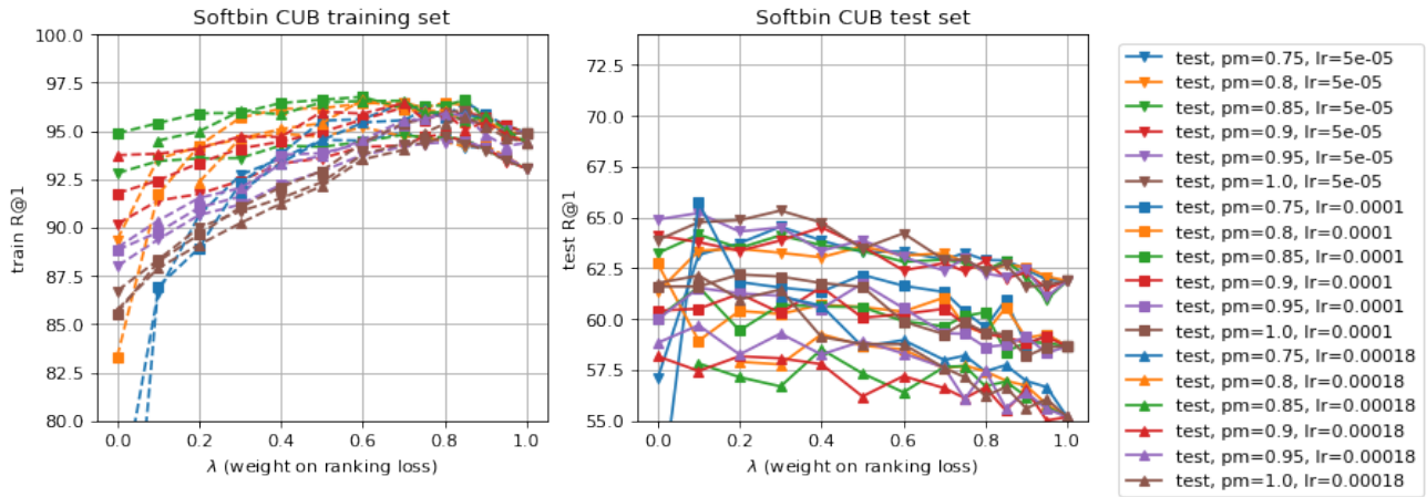
Figure 21. CUB R@1 results for Softbin-AP, with varying \lambda , learning rate, and positive margin on contrastive loss. We plot both train and test R@1 results. “lr” and “pm” in the legend stand for learning rate and positive margin \delta_+ , respectively.
