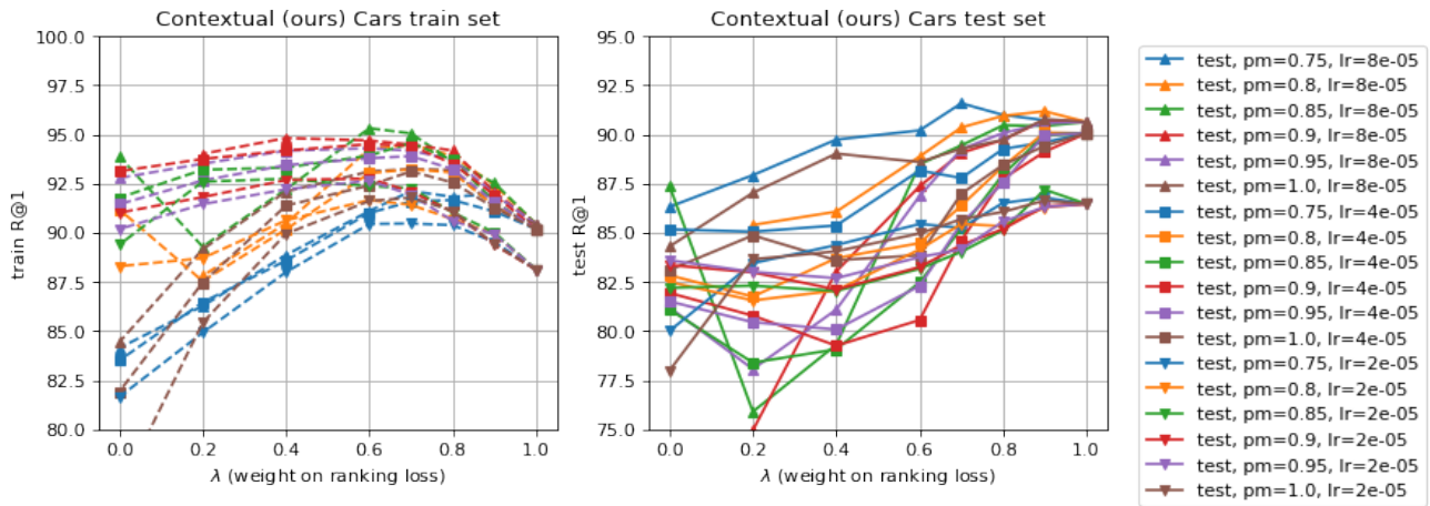
Figure 23. Cars R@1 results for our contextual loss function, with varying \lambda , learning rate, and positive margin on contrastive loss. We plot both train and test R@1 results. “lr” and “pm” in the legend stand for learning rate and positive margin \delta_+ , respectively.
