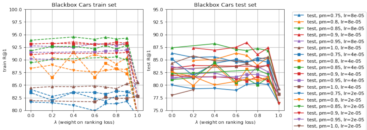
Figure 27. Cars R@1 results for Blackbox-AP, with varying \lambda , learning rate, and positive margin on contrastive loss. We plot both train and test R@1 results. “lr” and “pm” in the legend stand for learning rate and positive margin \delta_+ , respectively.
