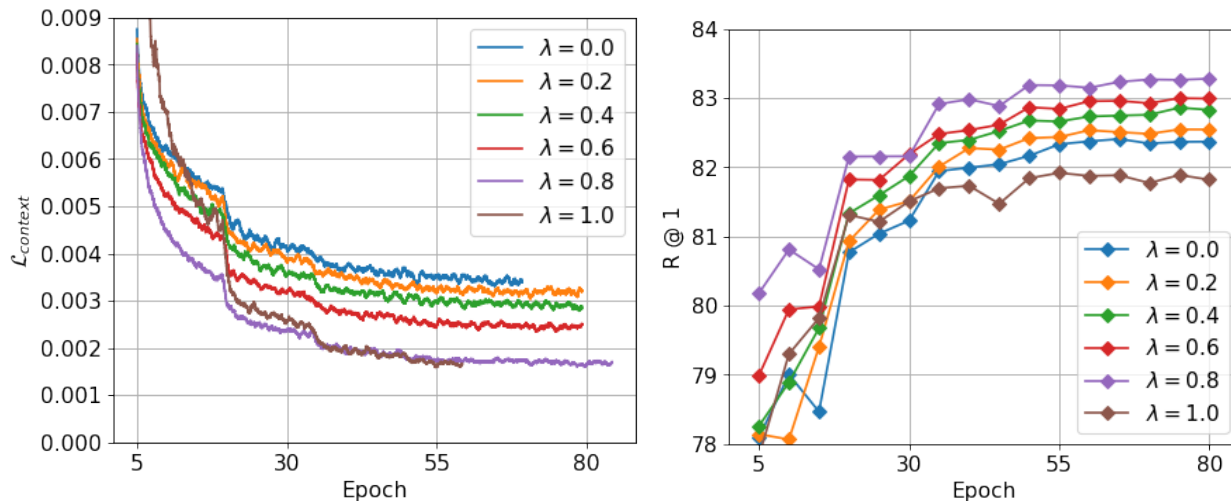
Figure 15. Plot of contextual similarity loss \mathcal{L}_{\text{context}} with varying \lambda . Each color is a different \lambda . Results are on the SOP dataset. Observe that the contrastive loss implicitly minimizes the contextual loss (blue line). Also observe that in general, a lower contextual loss corresponds to a higher test R@1. This shows that our loss function is a reasonable objective. Note that the plot on the left plots \mathcal{L}_{\text{context}} , not the complete training loss. \gamma = 0 .
