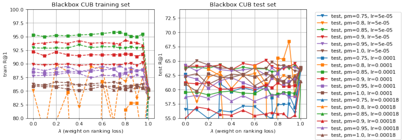
Figure 22. CUB R@1 results for Blackbox-AP, with varying \lambda , learning rate, and positive margin on contrastive loss. We plot both train and test R@1 results. “lr” and “pm” in the legend stand for learning rate and positive margin \delta_+ , respectively.
