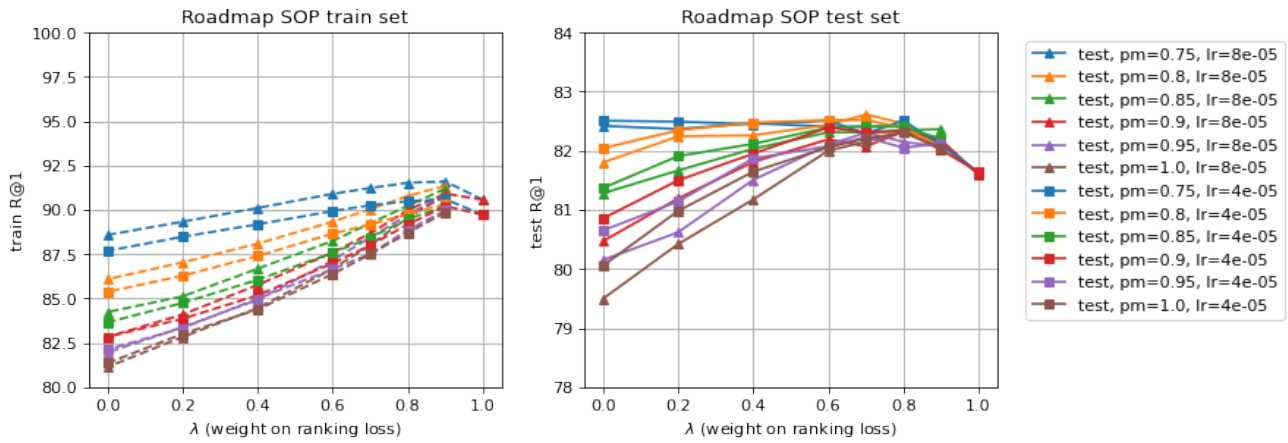
Figure 29. SOP R@1 results for Roadmap, with varying \lambda , learning rate, and positive margin on contrastive loss. We plot both train and test R@1 results. “lr” and “pm” in the legend stand for learning rate and positive margin \delta_+ , respectively.
