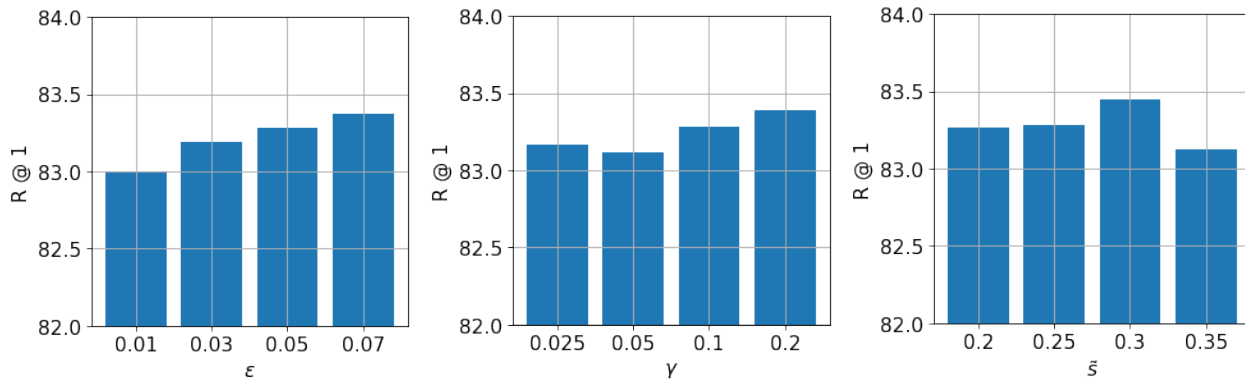
Figure 13. Hyperparameter tuning on SOP. We experiment with various values for \epsilon , \gamma and \tilde{s} . The R@1 values are similar for the different hyperparameter choices.
