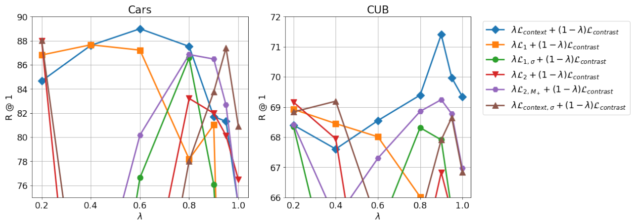
Figure 16. Ablation results on CUB and Cars. The blue line represents test R@1 of our framework for varying \lambda with \gamma = 0 . The other colors represent various modifications or simplifications of the loss function (reference Table 5 and Section F for full description). We perform each ablation experiment with varying \lambda since the optimal \lambda is not constant across all experiments. Clearly, the modified versions of \mathcal{L}_{context} are sub-optimal.
