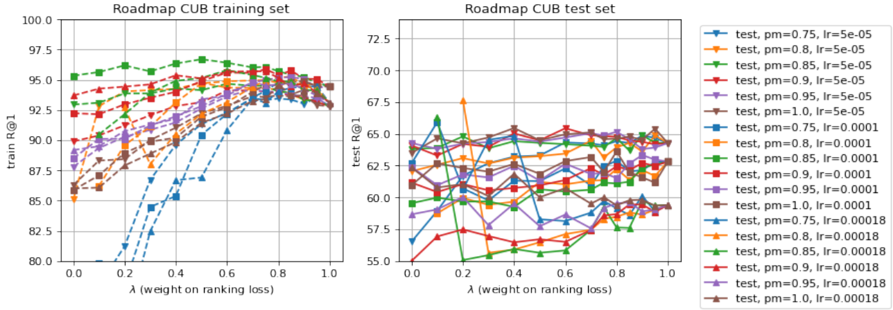
Figure 19. CUB R@1 results for Roadmap, with varying \lambda , learning rate, and positive margin on contrastive loss. We plot both train and test R@1 results. “lr” and “pm” in the legend stand for learning rate and positive margin \delta_+ , respectively.
