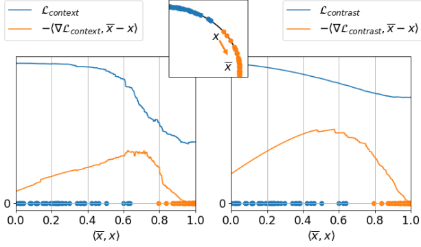
Figure 4. Illustration of \mathcal{L}_{\text{context}} and its gradient. We generate 64 random points on the unit circle from two classes, centered around the coordinates (0,1) and (1,0) (see middle plot). We move one orange point x from the blue centroid to the orange centroid \bar{x} . The value of the loss function is plotted in blue, and the amount of gradient pointing away from \bar{x} is plotted in orange. \mathcal{L}_{\text{context}} decreases as x rolls to the right, and the gradient closely approximates what it should look like if \mathcal{L}_{\text{context}} were continuous. We include the same illustration for \mathcal{L}_{\text{contrast}} on the right for comparison.
