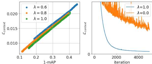
Figure 3. Left: plot of contextual loss value vs. 1-mAP (mean AP) over the course of training on CUB for different choices of \lambda . Training proceeds from upper right to bottom left. Observe that 1-mAP decreases as contextual loss decreases. This shows that \mathcal{L}_{\text{context}} is a valid surrogate for learning to rank. Right: convergence plot of \mathcal{L}_{\text{context}} on CUB without mini-batching. \mathcal{L}_{\text{context}} decreases almost monotonically when the contextual loss is minimized ( \lambda = 1 ), while there is a large amount of noise when the contrastive loss is minimized ( \lambda = 0 ). \gamma = 0 .
