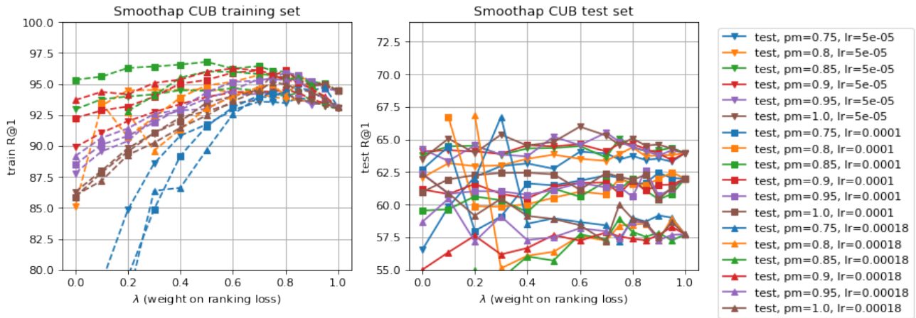
Figure 20. CUB R@1 results for Smooth-AP, with varying \lambda , learning rate, and positive margin on contrastive loss. We plot both train and test R@1 results. “lr” and “pm” in the legend stand for learning rate and positive margin \delta_+ , respectively.
