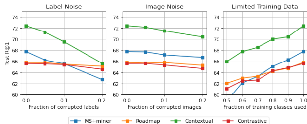
Figure 6. Robustness and generalizability comparison of the contextual loss against other pairwise ranking losses. See description in Section 4.4. For this experiment, we test \mathcal{L}_{\text{context}} without additional regularization, i.e. \lambda = 1 and \gamma = 0 .
