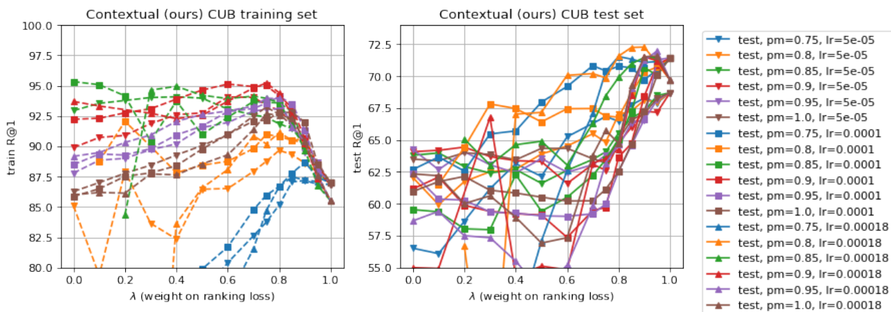
Figure 18. CUB R@1 results for our contextual loss function, with varying \lambda , learning rate, and positive margin on contrastive loss. We plot both train and test R@1 results. “lr” and “pm” in the legend stand for learning rate and positive margin \delta_+ , respectively.
