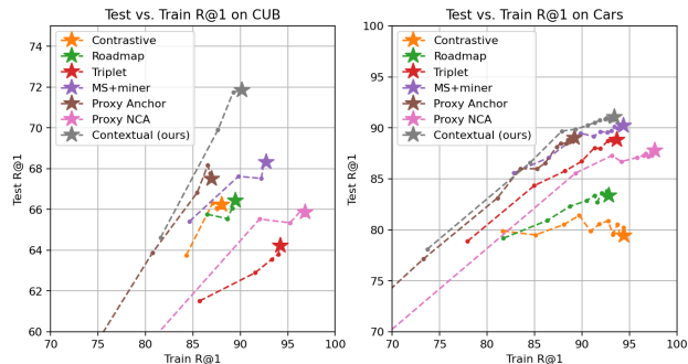
Figure 2. Comparison of our contextual loss with popular metric learning losses. We plot the test R@1 accuracy against the train R@1 accuracy over the course of training on the CUB and Cars benchmarks. The dashed line tracks the R@1 values over the course of training, and the star indicates the R@1 values at the end of training. Compared to baselines, the contextual loss achieves higher test R@1 at the expense of lower train R@1.
