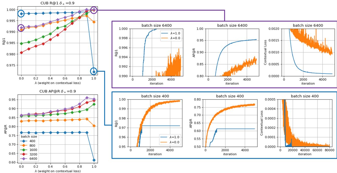
Figure 9. Empirical verification of the existence of a decomposability gap when optimizing the contextual loss. We run this experiment on CUB. We train the linear embedding layer on top of fixed ResNet-50 features. We experiment with different \lambda . \lambda = 0 corresponds to the contrastive loss, while \lambda = 1 corresponds to the contextual loss. We experiment with different batch sizes. We only plot the train R@1 accuracy in this figure. Note that batch size of 6400 corresponds to the entire dataset (i.e. decomposability gap is zero). The plots on the right show the R@1, AP@R, and contextual loss over the course of training for \lambda = 0 and \lambda = 1 for both the largest batch size and the smallest batch size. Observe that when the batch size is 400, optimizing the contextual loss ( \lambda = 1 ) in blue does not converge to the correct ranking on the entire dataset. The training stalls at around 1000 iterations. This is because the embedding space after iteration 1000 is good enough in the sense that the batch-wise ranking is perfect for all sampled batches. Meanwhile, if we use batch size 6400 (no mini-batching), the decomposability gap is zero, and the contextual loss in blue clearly converges to the correct ranking over the entire dataset. Further observe that on the larger batch sizes, the optimal train R@1 is achieved when \lambda = 1 . This suggests that the contrastive loss is not needed on large batch sizes, where the decomposability gap is smaller.
