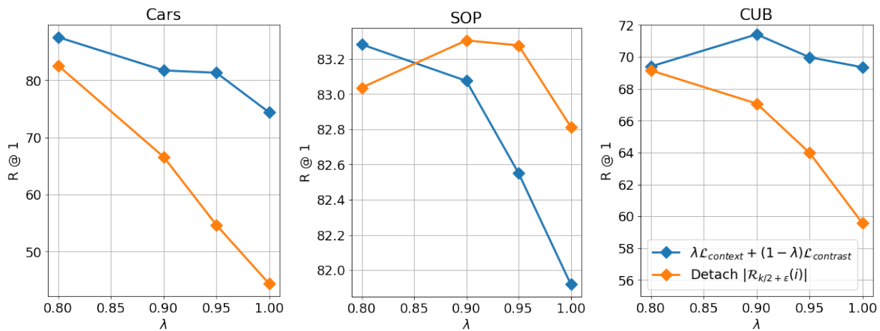
Figure 17. Investigating the effect of detaching |\mathcal{R}_{k/2+\epsilon}(i)| in Eq. 27. The blue line shows R@1 of our framework with varying \lambda . \gamma = 0 . The orange line shows R@1 after detaching |\mathcal{R}_{k/2+\epsilon}(i)| . Overall, detaching this normalization factor is undesirable.
