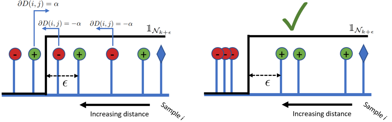
Figure 10. Illustration of \mathcal{N}_{k+\epsilon} optimization using the simplified loss function \mathcal{L}_1 in Eq. 32. Negative samples which are in the set \mathcal{N}_{k+\epsilon}(i) are pushed away from i by a constant gradient. Positive samples which are not in the set \mathcal{N}_{k+\epsilon}(i) are pulled closer. This behavior is analogous to the standard contrastive loss: \mathcal{L}_{\text{contrast}} applies a constant gradient to pairs violating a fixed margin, while \mathcal{L}_1 applies a constant gradient to pairs violating the flexible margin defined by the k -th neighbor. k = 4 in the illustration.
