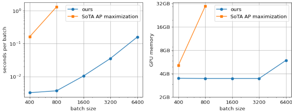
Figure 8. Comparison of scalability in time and space between our loss function and Roadmap. Our method is plotted in blue, while Roadmap is plotted in orange. For this experiment, we pre-calculate the 2048-dimensional ResNet-50 features and train a linear embedding layer using each loss function. Both the time taken per batch (left) and GPU memory used (right) scale cubically. However, the time and space taken to calculate our loss function is negligible compared to backbone evaluation, even for batch size 6400. On the other hand, the time and space needed to calculate the Roadmap loss quickly becomes unpractical for large batch sizes. Note: we pre-compute all features and store them in GPU memory. The memory used by the pre-computation is freed, but the GPU memory being used, as indicated by the Nvidia tool, remains at the maximum memory used over the lifetime of the process. Therefore, the memory consumed by calculating the loss function is not visible until it exceeds the memory used by the pre-computation.
