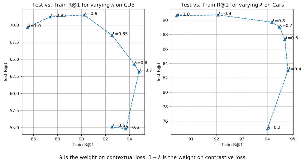
Figure 14. Test R@1 vs. train R@1 accuracy for varying \lambda ( \gamma = 0 ). This figure shows that adding the standard contrastive loss (lowering \lambda ) increases the R@1 on training data. This also increases the test R@1 up to a point (approximately \lambda = 0.9 ), before overfitting.
