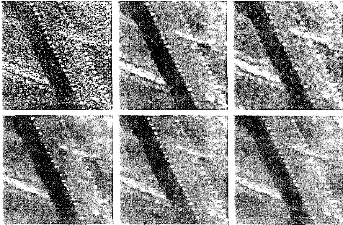
Figure 10: Comparison of speckle noise reduction methods. (a) Top Left: SAR image (compressed for viewing) of scene with overpass over New York State Thruway, taken from image in Figure 1. (b) Top Middle: Multi-scale BCS/ECS. (c) Top Right: 3 iterations of 3x3 median filter. (d) Bottom Left: Adaptive averaging using 2 iterations of 5x5 sigma filter. (e) Bottom Middle: 3 iterations of geometric filter. (f) Bottom Right: 1 iterations of geometric filter.
