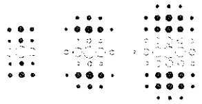
Figure 12: (a): Horizontal bipole filters at three spatial scales. The length of each oriented line segment is proportional to the filter coefficient at that location and orientation. (b): Horizontal feedback intra-orientational spatial sharpening filters at three spatial scales.
