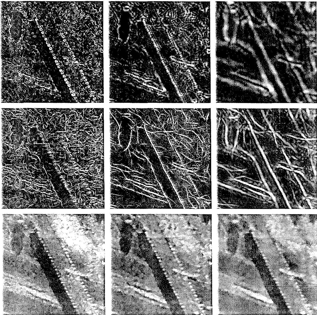
Figure 10: Top Row: Stage 3 complex cell processing at three scales of Model II. Intensity of each pixel depicts the total activity of the oriented complex cells at that position. Middle Row: Stage 5 hypercomplex cell processing at three spatial scales. Intensity of each pixel depicts the total activity of the cells at that position. Bottom Row: Stage 9 processing result at three different scales on example image. A linear combination of these images is used to obtain the final multiple-scale output in Figure 14.
