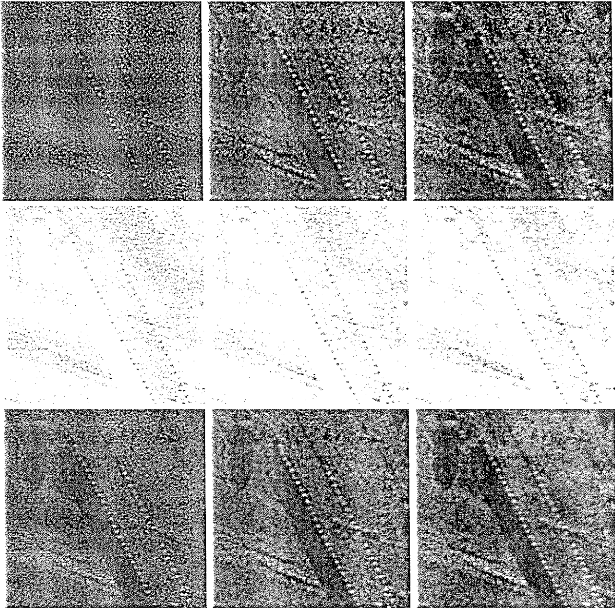
Figure 7: In Model II: (a) Rectified ON cell responses at small, medium, and large scales from left to right. (b) Rectified OFF cell responses. (c) Double-opponent ON-minus-OFF responses.
