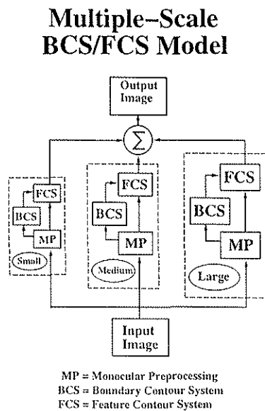
Figure 4: A multiple-scale BCS/FCS model.
