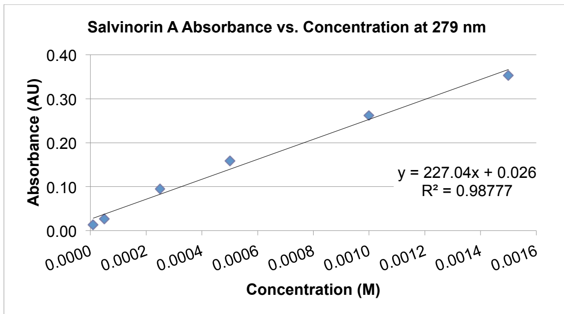
Figure 17. Salvinorin A absorbance versus concentration at 279 nm. The molar absorptivity at 279 nm is 227.04 \text{ M}^{-1}\text{cm}^{-1} .
