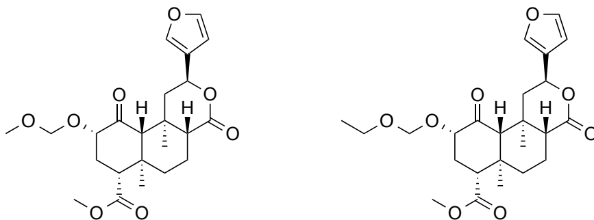
Salvinorin B Methoxymethyl Ether Salvinorin B Ethoxymethyl Ether
