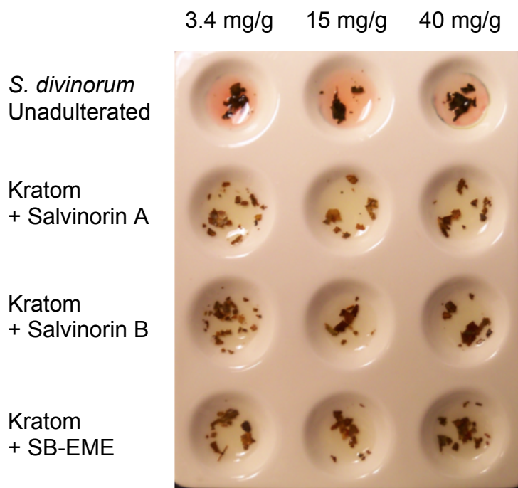
Figure 39. Adulterated Kratom with salvinorin A, salvinorin B, and SB-EME after reaction with Ehrlich's reagent. After 2 min, the adulterated samples showed a negative result. The top row contained 3 replicates of unadulterated S. divinorum as a control. Each column contains 3.4, 15, or 40 mg/g of spiking standard, respectively.
