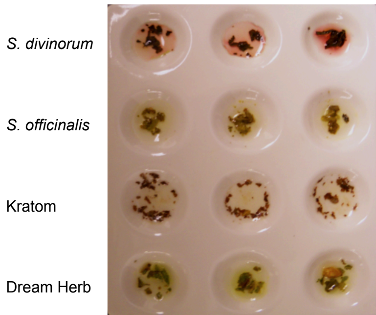
Figure 35. Samples of unadulterated S. divinorum , S. officinalis , Kratom, and Dream Herb after reaction with Ehrlich's reagent. Samples reacted for 2 min (n = 3).
