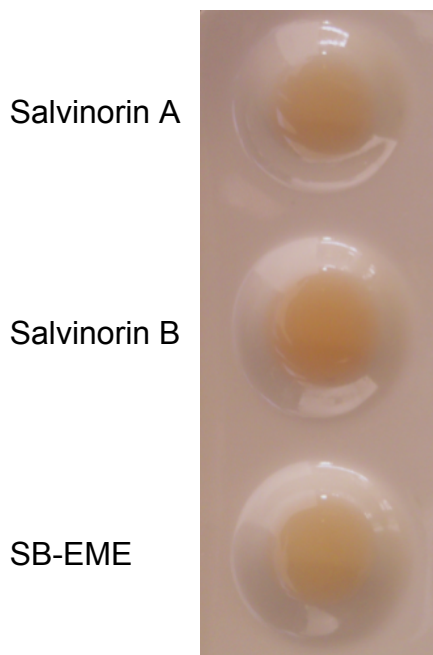
Figure 33. Colorimetric analysis of salvinorin A, salvinorin B, and SB-EME standards. Standards of 1 mmol/L were analyzed and allowed to react for 2 min prior to photograph.
