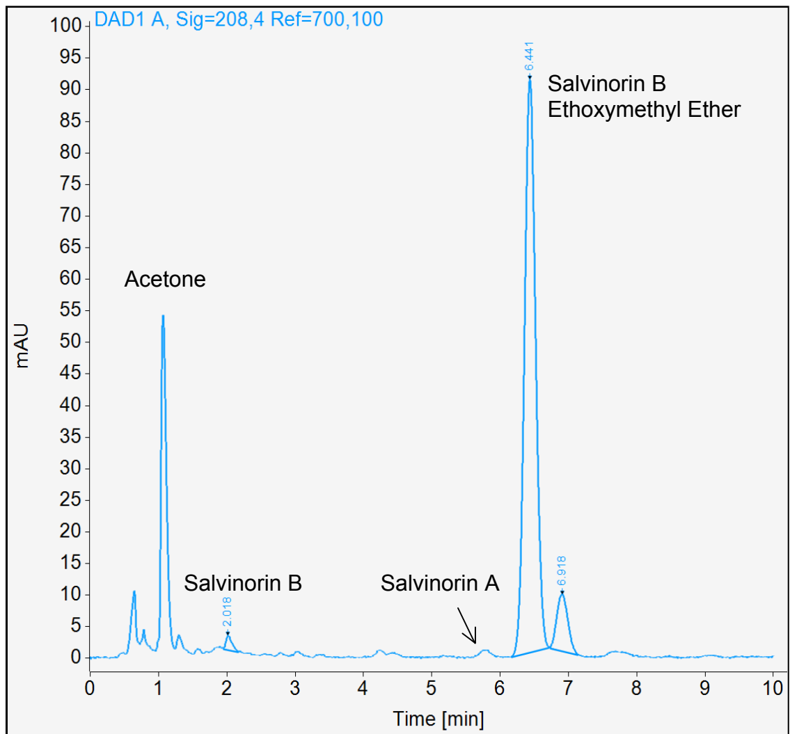
Figure 12. HPLC trace of SB-EME at 4.8 µg. The RT of SB-EME is 6.44 min, achieving baseline resolution from salvignorin A, salvignorin B, and other impurities.
