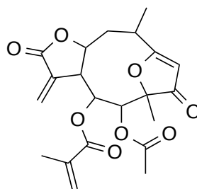
Figure 36. Structure of 9 \alpha -acetoxyzexbrevin from Dream Herb. Stereochemistry not indicated.
