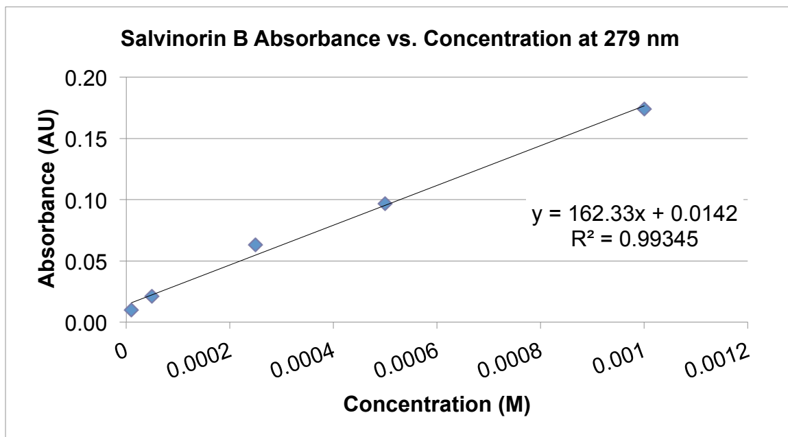
Figure 18. Salvinorin B absorbance versus concentration at 279 nm. The molar absorptivity at 279 nm is 162.33 \text{ M}^{-1}\text{cm}^{-1} .
