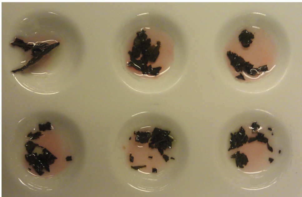
Figure 20. Salvia divinorum after addition of Ehrlich's reagent. Photograph was taken after 2 minutes of reaction (n=6).
