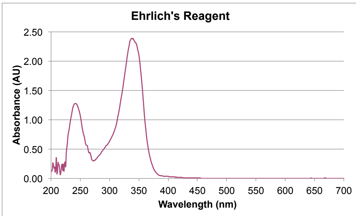
Figure 28. UV/Vis of Ehrlich's reagent. 1:10 dilution in ethanol.
